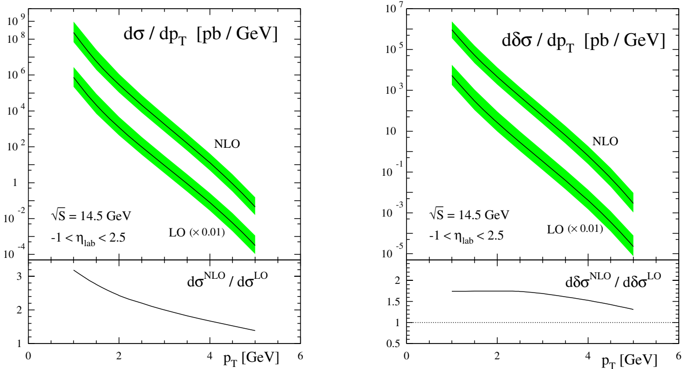
FIG. 3 (color online). Unpolarized (left) and transversely polarized (right) single-inclusive neutral-pion production cross sections at LO and NLO at the GSI. The LO results have been scaled by a factor of 0.01. The shaded bands represent the theoretical uncertainty if the factorization/renormalization scale \mu is varied in the range p_T \leq \mu \leq 4p_T . The lower panel shows the ratios of the NLO and LO results in each case, using \mu = 2p_T .
