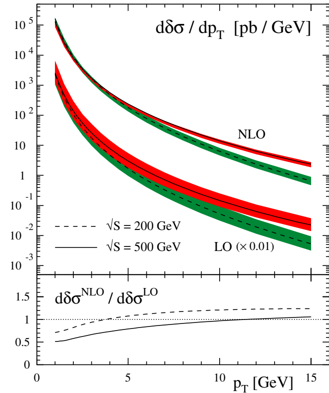
FIG. 1 (color online). Transversely polarized single-inclusive neutral-pion production cross sections in LO and NLO for \sqrt{S} = 200 and 500 GeV collisions at RHIC. The LO results have been scaled by a factor of 0.01. The shaded bands represent the changes if the scale \mu is varied in the range p_T \leq \mu \leq 4p_T . The lower panel shows the ratios of the NLO and LO results for both c.m.s. energies.
