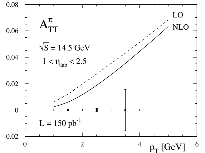
FIG. 4. Upper bounds for the transverse double-spin asymmetry A_{TT} for single-inclusive neutral-pion production in LO and NLO at GSI-FAIR. The “error bars” indicate the expected statistical accuracy for bins in p_T (see text).
