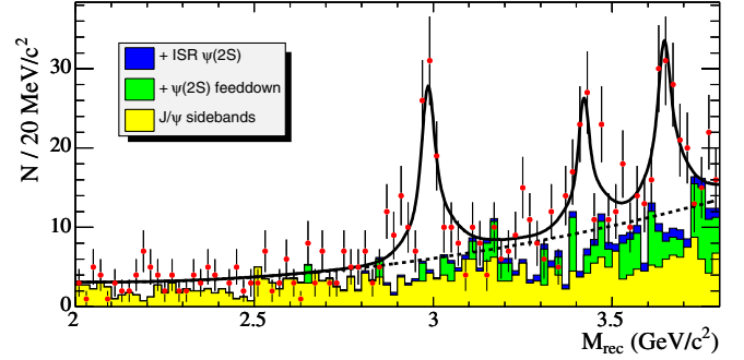
FIG. 2 (color online). The fit to the recoil mass distribution is represented by the solid curve. The dashed curve is a second-order polynomial representing the background. The points with error bars refer to the events in the J/\psi mass window. The histograms represent different sources of backgrounds.
