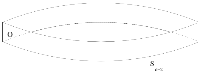
FIG. 3. A space S_{d-1} = O \times S_{d-2} , where O is an orbifold (interval).
