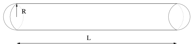
FIG. 1. A sausagelike manifold leading to topologically trivial vacuum and to the absence of the \theta problem.
