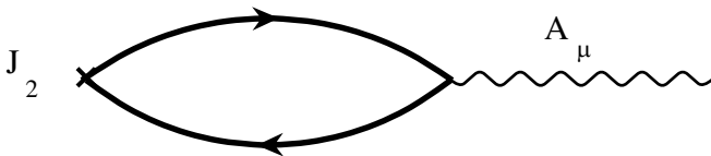
FIG. 4. The Feynman that gives a nonzero contribution to the current through the end points of the interval.
