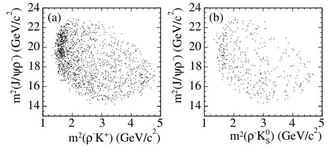
FIG. 2. The m^2(J/\psi \rho^-) versus the m^2(\rho^- K^+) distributions (a) for B^0 \rightarrow J/\psi \pi^- \pi^0 K^+ and the m^2(J/\psi \rho^-) versus the m^2(\rho^- K_S^0) distributions (b) for B^- \rightarrow J/\psi \pi^- \pi^0 K_S^0 . A B \rightarrow J/\psi K_1 signal can be seen; however, there is no indication for an enhancement in the J/\psi \rho^- mass spectrum.
