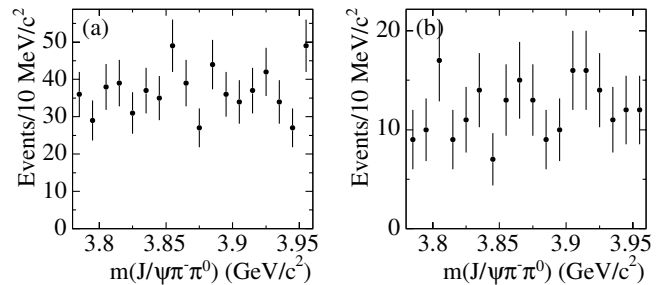
FIG. 3. The J/\psi \pi^- \pi^0 invariant mass in 10 \text{ MeV}/c^2 bins for (a) B^0 \rightarrow J/\psi \pi^- \pi^0 K^+ and (b) for B^- \rightarrow J/\psi \pi^- \pi^0 K_S^0 . No indication for the decay X^- \rightarrow J/\psi \pi^- \pi^0 can be found.
