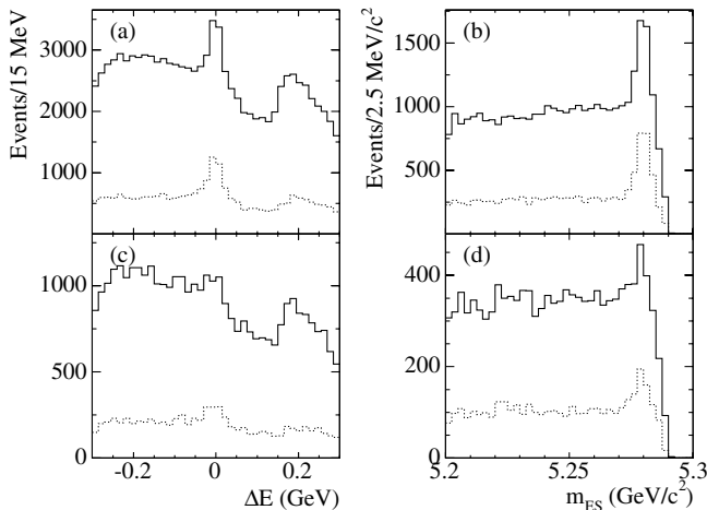
FIG. 1. The \Delta E (a) and m_{ES} (b) distributions for the B^0 \rightarrow J/\psi \pi^- \pi^0 K^+ mode and the \Delta E (c) and m_{ES} (d) distributions for the B^- \rightarrow J/\psi \pi^- \pi^0 K_S^0 mode using the optimized cuts. The dotted line shows the same with the additional cut 0.67 < m(\pi^- \pi^0) < 0.87 \text{ GeV}/c^2 .
