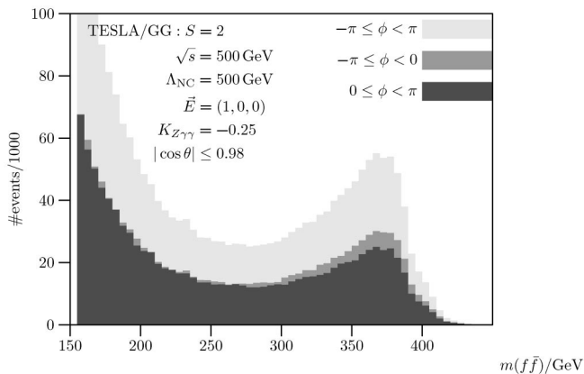
FIG. 5. Number of events per year in the two half-spheres \phi < 0 and \phi > 0 for \sqrt{s} = 500 GeV.
