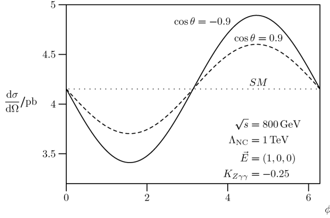
FIG. 1. Dependence of the differential NCSM cross section on the azimuthal angle \phi for the timelike noncommutativity \vec{E} perpendicular to the beam axis.
