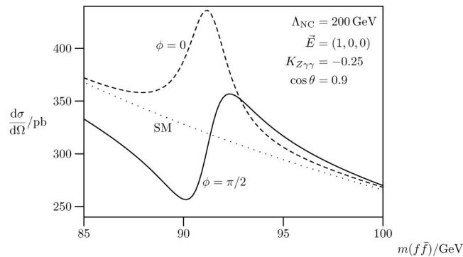
FIG. 2. The interference of the SM and \mathcal{O}(\theta) NCSM amplitudes around the Z resonance is plotted for different values of the azimuthal angle \phi .
