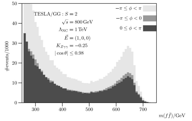
FIG. 3. Number of events per year in the two half-spheres \phi < 0 and \phi > 0 for \sqrt{s} = 800 \text{ GeV} .
