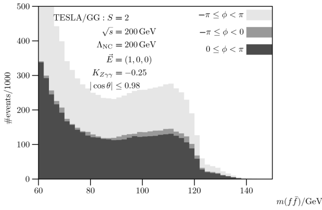
FIG. 4. Number of events per year in the two half-spheres \phi < 0 and \phi > 0 for \sqrt{s} = 200 GeV.
