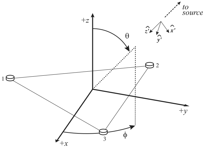
FIG. 3. The array and the wave coordinates. The x , y , and z axes are the LISA coordinate axes with the origin at the point o , and the array lies in the x , y plane. The x' , y' , z' axes are the coordinate axes for the incoming gravitational wave. The z' axis is parallel to the direction of propagation of the wave. The x' , y' axes are those with respect to which h_+(t) and h_\times(t) are defined. The angles \theta , \phi describe the location of the source in the sky.
