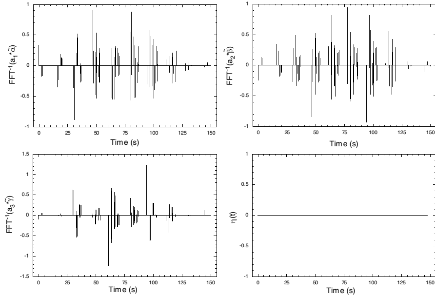
FIG. 7. Plots (a)–(d) are as in Fig. 6, but now with (\theta = \theta_s, \phi = \phi_s) .
