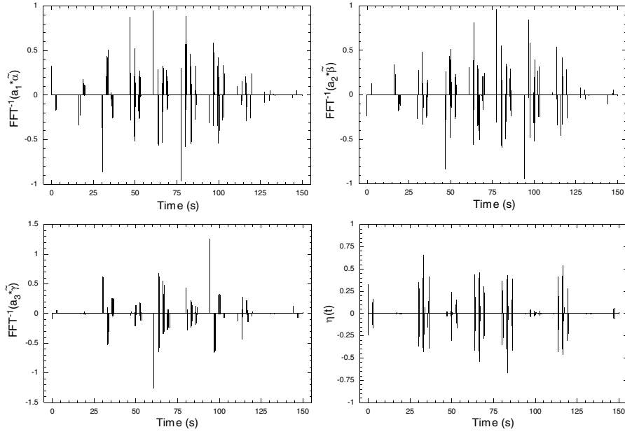
FIG. 6. The time-domain responses of the inverse-Fourier transforms of the three functions, a_1\tilde{\alpha} (a), a_2\tilde{\beta} (b), a_3\tilde{\gamma} (c), which determine the ZSS. The angles (\theta, \phi) , over which the search is performed have been fixed to be equal to \theta = 31.5^\circ , \phi = 106.5^\circ ; (d) the ZSS constructed from the functions shown in (a)–(c).
