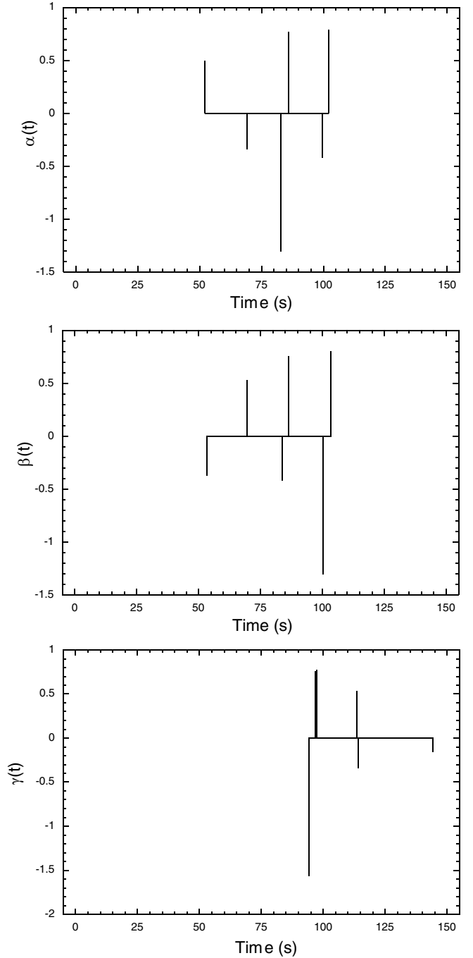
FIG. 5. The responses of the three Sagnac combinations, \alpha (a), \beta (b), and \gamma (c), to a gravitational wave burst of unit amplitudes. The source has been assumed to be located at \theta_s = 32^\circ , \phi_s = 107^\circ .
