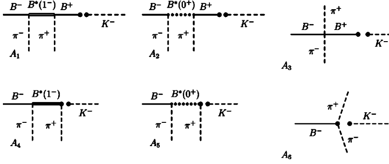
FIG. 1. Feynman diagrams contributing to the nonresonant part of the amplitude.
