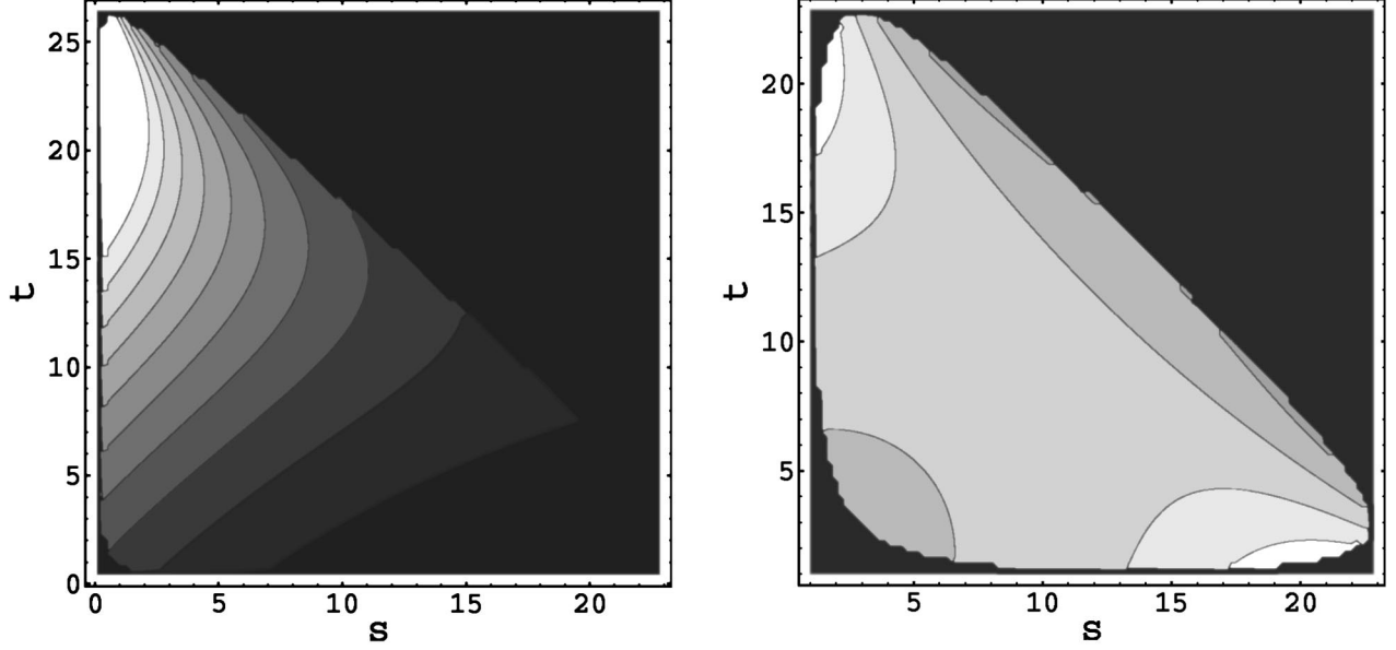
FIG. 2. Dalitz plots for the nonresonant B^- \rightarrow K^- \pi^- \pi^+ (left) and B^- \rightarrow K^- K^- K^+ (right) decay modes.
