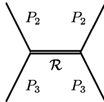
FIG. 4. Rescattering of the P_2 and P_3 states through the resonance \mathcal{R} .
