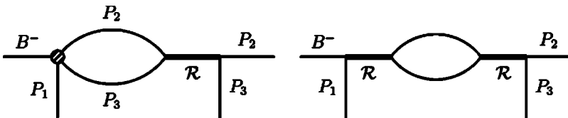
FIG. 3. Diagrams presenting the nonresonant (left) and the resonant (right) contributions to dispersive part of the amplitude in the phase space region of the P_2 and P_3 invariant mass close to the \mathcal{R} mass. Blob in the left diagram presents the nonresonant weak decay mode (see Fig. 1).
