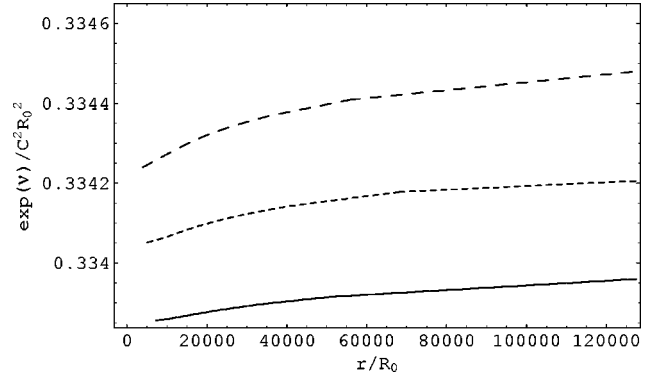
FIG. 2. Variation, as a function of the parameter r/R_0 , of the metric coefficient \exp(\nu)/C^2 R_0^2 for a static, conformally symmetric vacuum space-time on the brane, for B = 1.00001 and different values of k : k=0.9999 (solid curve), k = 0.99985 (dotted curve), and k=0.9998 (dashed curve).
