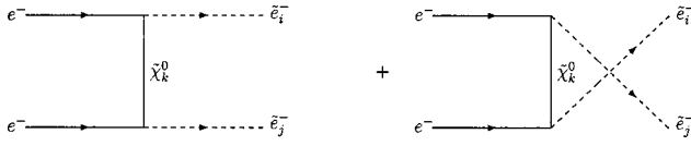
FIG. 8. Diagrams for e^- e^- \rightarrow \tilde{e}_i^- \tilde{e}_j^- .
