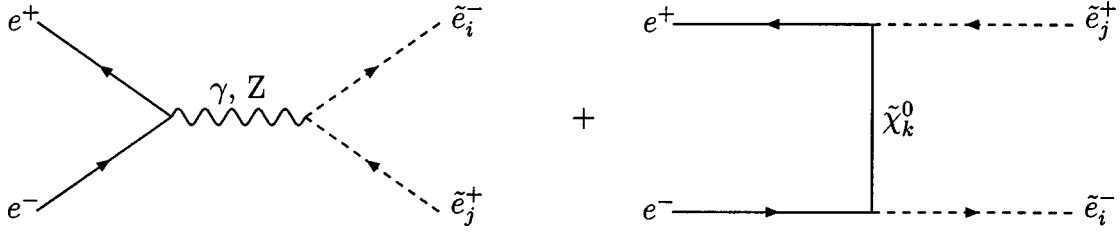
FIG. 7. Diagrams for e^+e^- \rightarrow \tilde{e}_i^- \tilde{e}_j^+ .
