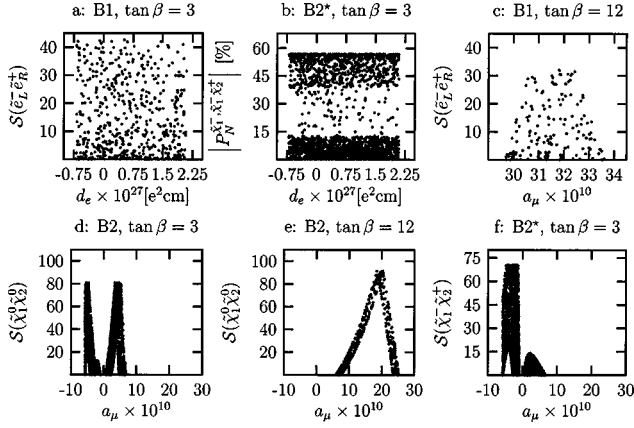
FIG. 11. Correlations between low- and high-energy quantities. Most high-energy observables have been computed at \sqrt{s} = 500 GeV, except for panels (b) and (f), which are for \sqrt{s} = 800 GeV. The parameter sets B1 and B2 have been defined in Table I, and the significance S is defined via Eq. (6.2).
