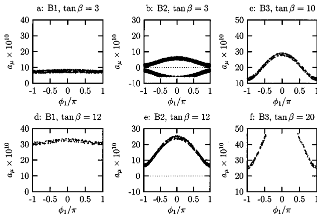
FIG. 5. (a_\mu)_{\text{SUSY}} vs \phi_1 after scanning over \phi_\mu and \phi_A .
