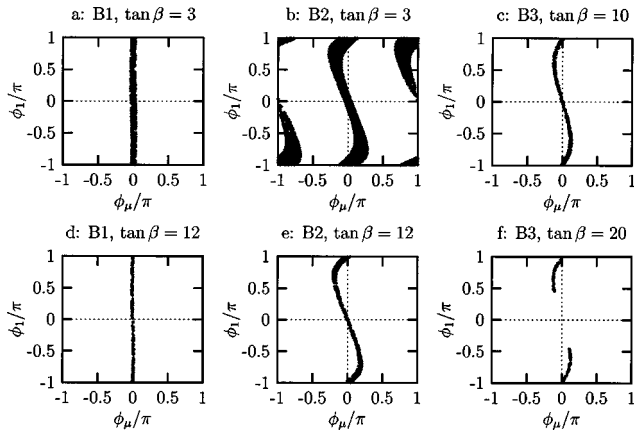
FIG. 2. Combinations of \phi_\mu and \phi_1 that are allowed for at least one \phi_A \in [-\pi, \pi] .
