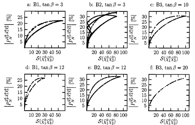
FIG. 14. Correlation between the significance \mathcal{S} and the absolute value of normal polarization P_N , measured at scattering angle \theta = \pi/2 , for mixed neutralino pair production at \sqrt{s} = 500 GeV. We consider \tilde{\chi}_1^0 \tilde{\chi}_2^0 production for scenarios B2 and B3, but switch to the \tilde{\chi}_1^0 \tilde{\chi}_3^0 final state for scenario B1.
