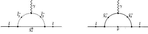
FIG. 1. SUSY contributions to leptonic dipole operators.
