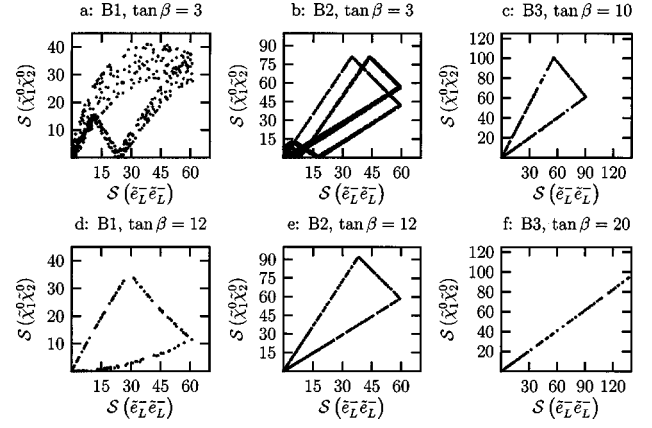
FIG. 12. Correlations between the significances, defined as in Eq. (6.2), for the processes e^-e^- \rightarrow \tilde{e}_L^- \tilde{e}_L^- and e^+e^- \rightarrow \tilde{\chi}_1^0 \tilde{\chi}_2^0 , both taken at \sqrt{s} = 500 GeV.
