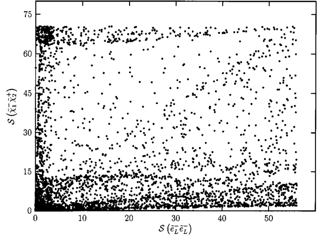
FIG. 13. Correlation between the significances for the processes e^- e^- \rightarrow \bar{e}_L^- \bar{e}_L^- and e^+ e^- \rightarrow \tilde{\chi}_1^- \tilde{\chi}_2^+ , both taken at \sqrt{s} = 800 GeV, for scenario B2 with \tan \beta = 3 .
