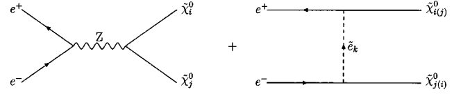
FIG. 10. Diagrams for e^- e^+ \rightarrow \tilde{\chi}_i^0 \tilde{\chi}_j^0 .
