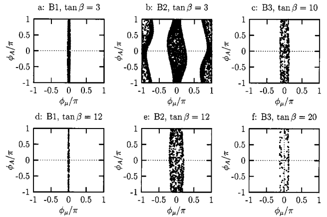
FIG. 3. Combinations of \phi_\mu and \phi_A that are allowed for at least one value of \phi_1 \in [-\pi, \pi] .
