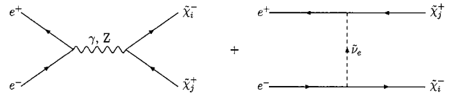
FIG. 9. Diagrams for e^- e^+ \rightarrow \tilde{\chi}_i^- \tilde{\chi}_j^+ .
