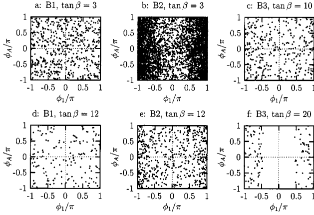
FIG. 4. Combinations of \phi_1 and \phi_A that are allowed for at least one value of \phi_\mu \in [-\pi, \pi] .
