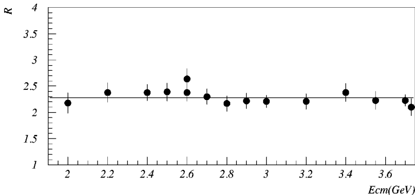
FIG. 1. R measurements in the c.m. energy range from 2.0 to 3.73 GeV from BES [5] with best fit R = 2.28 \pm 0.04 .
