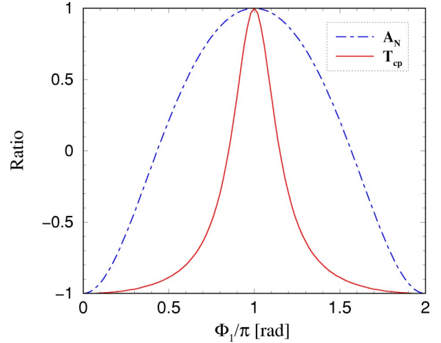
FIG. 3. The dependence of the ratio \mathcal{T}_{CP} (solid line) and the asymmetry \mathcal{A}_N (dot-dashed line) on the CP phase \Phi_1 for the set of real parameters, \{\tan\beta=10, M_2=250 \text{ GeV}, |\mu|=500 \text{ GeV}\} . The phase \Phi_\mu is set zero in this numerical illustration figure, as the ratio \mathcal{T}_{CP} and the asymmetry \mathcal{A}_N are found to be insensitive to the phase \Phi_\mu for the given specific set of real parameters.
