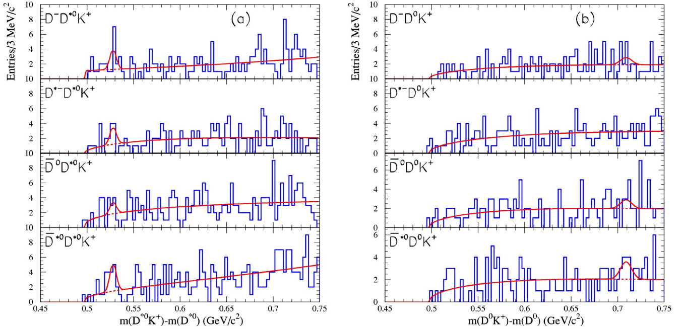
FIG. 6. (a) \Delta m = m(D^{*0}K^+) - m(D^{*0}) distributions of the events reconstructed in the four B \rightarrow \bar{D}^{(*)}D^{*0}K^+ decay modes, with 5.27 < m_{\text{ES}} < 5.29 \text{ GeV}/c^2 . (b) \Delta m = m(D^0K^+) - m(D^0) distributions of the events reconstructed in the four B \rightarrow \bar{D}^{(*)}D^0K^+ decay modes, with 5.27 < m_{\text{ES}} < 5.29 \text{ GeV}/c^2 . These distributions are fit with the sum of a threshold function g [Eq. (9)] for the background components and a Gaussian function for the D_{s1}(2536) and D_{sJ}(2573) components. The mean value and standard deviation of the Gaussian distributions have been fixed to the values obtained from a fit to the inclusive D_{s1}(2536) and D_{sJ}(2573) samples, as described in the text.
