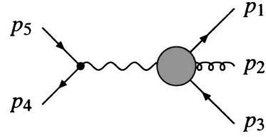
FIG. 1. Labeling of the external legs for the amplitude. The lepton pair is denoted by p_4 and p_5 .
