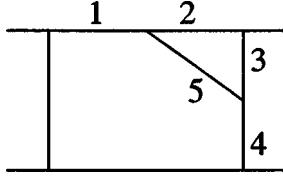
FIG. 2. The PentaBox represents a typical diagram where the triangle relation can be applied. In the present calculation, the lower left leg is massive.
