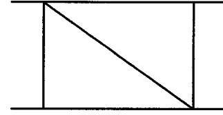
FIG. 3. The generic CBox. For the CBox 2 , the upper right external leg is massive.
