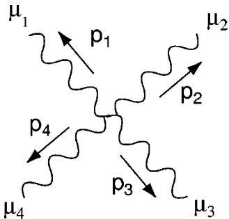
FIG. 1. Four-photon vertex.
