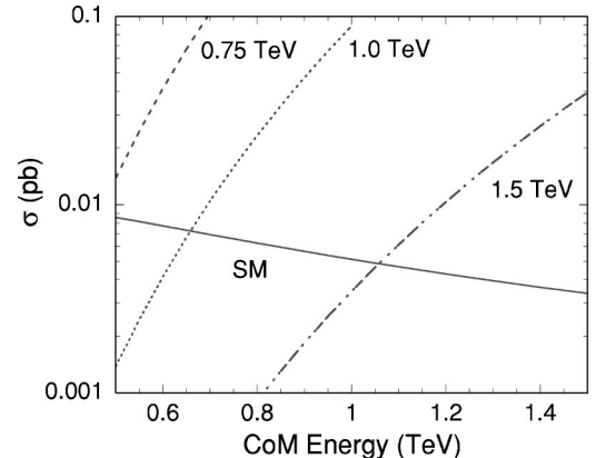
FIG. 2. Total crosssections \sigma_{\text{NC}} and \sigma_{\text{SM}} for 30^\circ < \Theta^* < 150^\circ . Noncommutative results are labeled by the value of \Lambda_{\text{NC}} , defined in the text.
