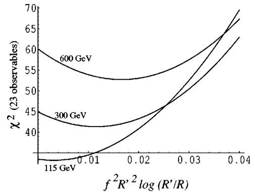
FIG. 1. The change in \chi^2 in the RS model as a function of R' and R , for three different values of M_H = 115, 300, and 600 GeV.
