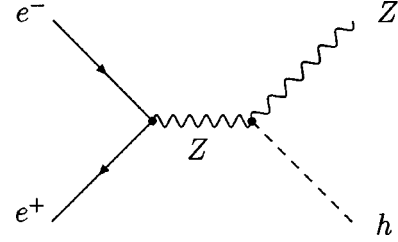
FIG. 1. Feynman diagram for the lowest order contribution to e^+e^- \rightarrow hZ .
