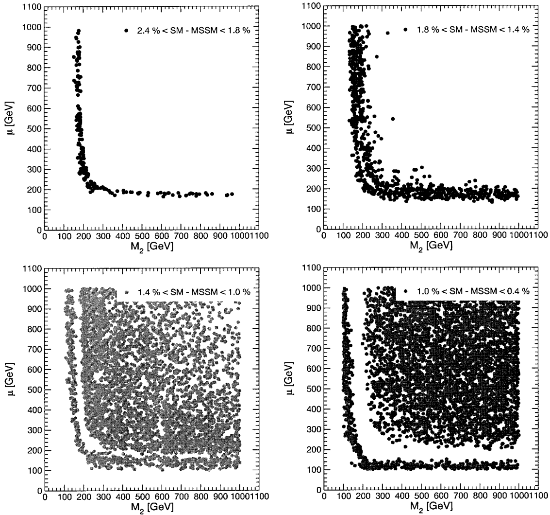
FIG. 3. The deviation of \sigma_{hZ}^{\text{SUSY}} from \sigma_{hZ}^{\text{SM}} = 0.1530 pb is shown in the M_2 - \mu -plane for M_h = 115 \pm 0.5 GeV at \sqrt{s} = 350 GeV with \mathcal{L} = 500 \text{ fb}^{-1} .
