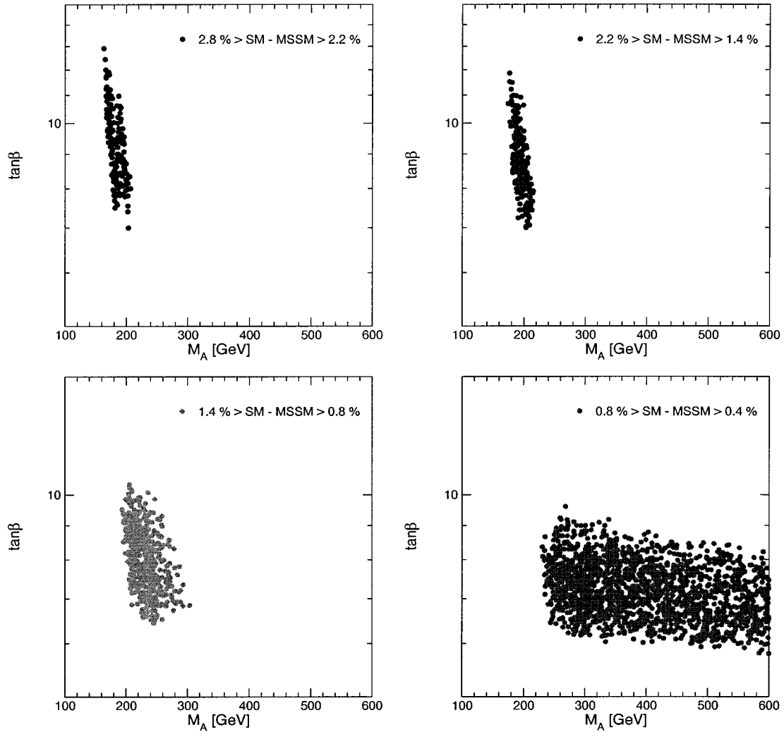
FIG. 2. The deviation of \sigma_{hZ}^{\text{SUSY}} from \sigma_{hZ}^{\text{SM}} = 0.1530 pb is shown in the M_A - \tan \beta -plane for M_h = 115 \pm 0.5 GeV at \sqrt{s} = 350 GeV with \mathcal{L} = 500 \text{ fb}^{-1} . For the \tilde{t} sector we have assumed the LC errors in Eq. (11).
