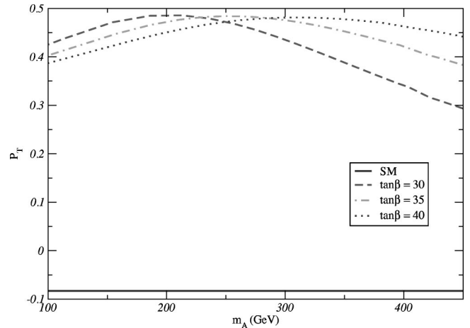
FIG. 10. P_T vs m_A for B_s \rightarrow \tau^+ \tau^- \gamma at \hat{s}=0.68 in SUGRA, other parameters are m=200 GeV, M=450 GeV, and A=0 .
