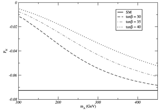
FIG. 9. P_N vs m_A at \hat{s}=0.68 for B_s \rightarrow \tau^+ \tau^- \gamma in SUGRA, other parameters are m=200 GeV, M=450 GeV, and A=0 .
