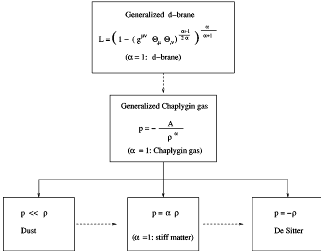
FIG. 1. Cosmological evolution of a universe described by a generalized Chaplygin gas equation of state.
