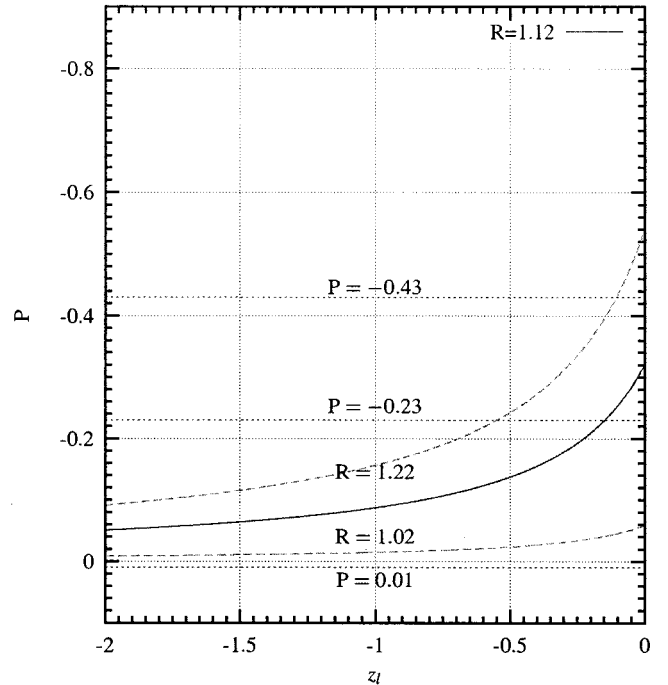
FIG. 2. The plot of P vs z_l is shown by employing the ALEPH ratio R = 1.12 \pm 0.10 . The experimental polarization P = -0.23^{+0.24}_{-0.20} is also shown to indicate the allowed range of z_l .
