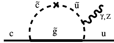
FIG. 9. A typical contribution to c \rightarrow u FCNC transitions in the MSSM. The cross denotes one mass insertion (\delta_{12}^u)_{\lambda\lambda'} , with \lambda, \lambda' = L, R .
