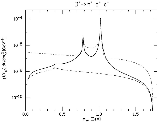
FIG. 1. The dilepton mass distribution for D^+ \rightarrow \pi^+ e^+ e^- , normalized to \Gamma_{D^+} . The solid line shows the sum of the short and the long distance SM contributions. The dashed line corresponds to the short distance contribution only. The dot-dash line includes the allowed R -parity violating contribution from supersymmetry (see Sec. III A 2).
