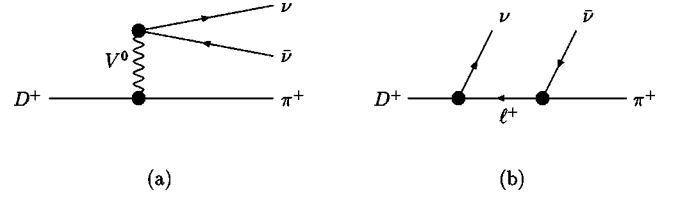
FIG. 3. Some long distance contributions.
