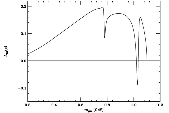
FIG. 14. The lepton forward-backward asymmetry for D^0 \rightarrow \rho^0 \mu^+ \mu^- for the bound of Eq. (78) (see text for details).
