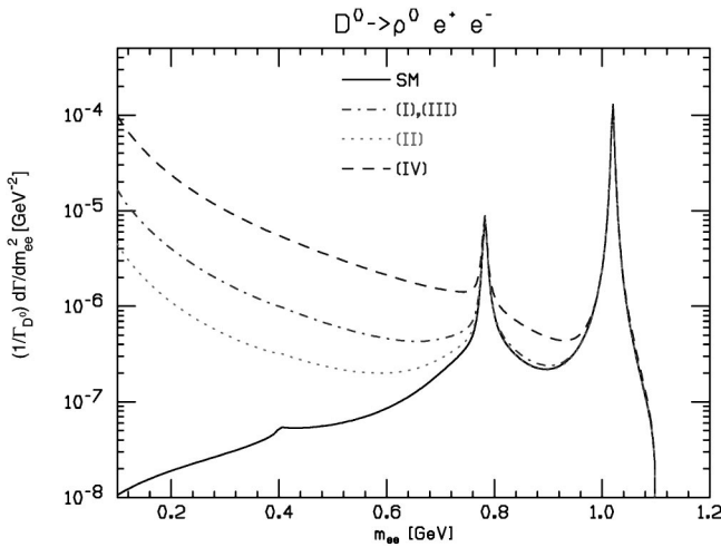
FIG. 11. The dilepton mass distribution for D \rightarrow \rho^0 e^+ e^- (normalized to \Gamma_{D^0} ) in the MSSM with non-universal soft breaking effects. The solid line is the SM; (I) M_{\tilde{g}} = M_{\tilde{q}} = 250 GeV; (II) M_{\tilde{g}} = 2 M_{\tilde{q}} = 500 GeV; (III) M_{\tilde{g}} = M_{\tilde{q}} = 1000 GeV and (IV) M_{\tilde{g}} = (1/2) M_{\tilde{q}} = 250 GeV.
