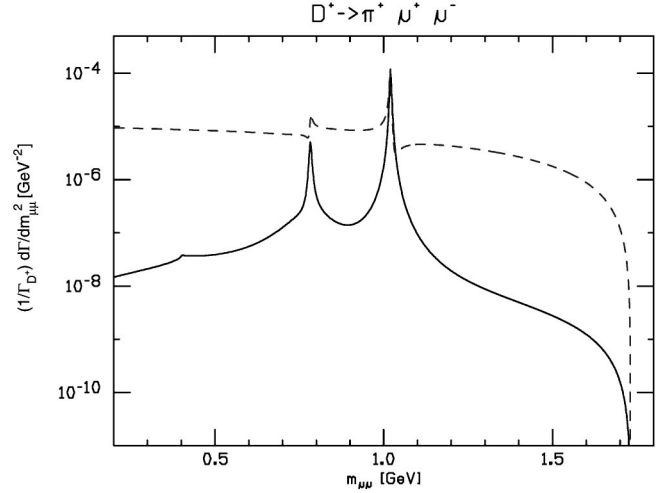
FIG. 12. The dilepton mass distribution for D^+ \rightarrow \pi^+ \mu^+ \mu^- normalized to \Gamma_{D^+} . The solid line shows the sum of the short and the long distance SM contributions. The dashed line includes the allowed R -parity violating contribution from supersymmetry (see text for details).
