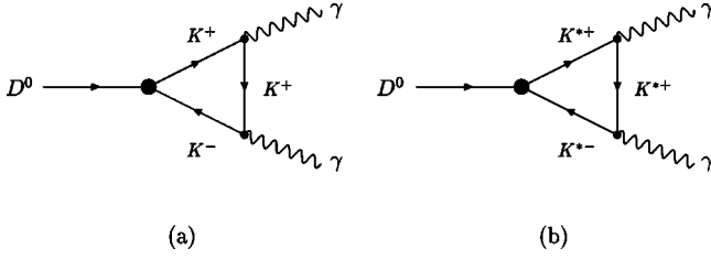
FIG. 7. Unitarity contributions: (a) K^+K^- , (b) K^{*+}K^{*-} .
