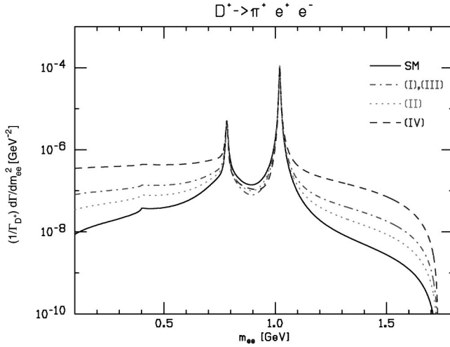
FIG. 10. The dilepton mass distribution for D^+ \rightarrow \pi^+ e^+ e^- (normalized to \Gamma_{D^+} ) in the MSSM with non-universal soft breaking effects. The solid line is the SM; (I) M_{\tilde{g}} = M_{\tilde{q}} = 250 GeV; (II) M_{\tilde{g}} = 2 M_{\tilde{q}} = 500 GeV; (III) M_{\tilde{g}} = M_{\tilde{q}} = 1000 GeV and (IV) M_{\tilde{g}} = (1/2) M_{\tilde{q}} = 250 GeV.
