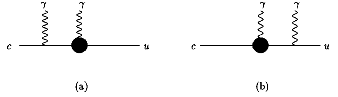
FIG. 4. 1PR contributions to c \rightarrow u \gamma \gamma .
