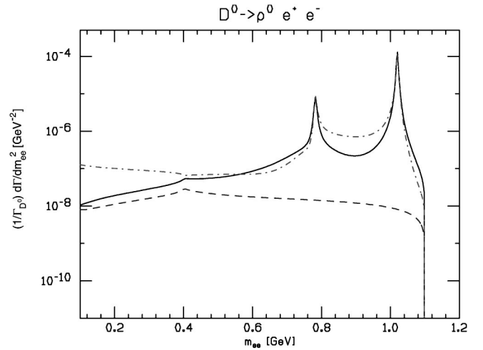
FIG. 2. The dilepton mass distribution for D^0 \rightarrow \rho^0 e^+ e^- , normalized to \Gamma_{D^0} . The solid line shows the sum of the short and the long distance SM contributions. The dashed line corresponds to the short distance contribution only. The dot-dash line includes the allowed R -parity violating contribution from supersymmetry (see Sec. III A 2).
