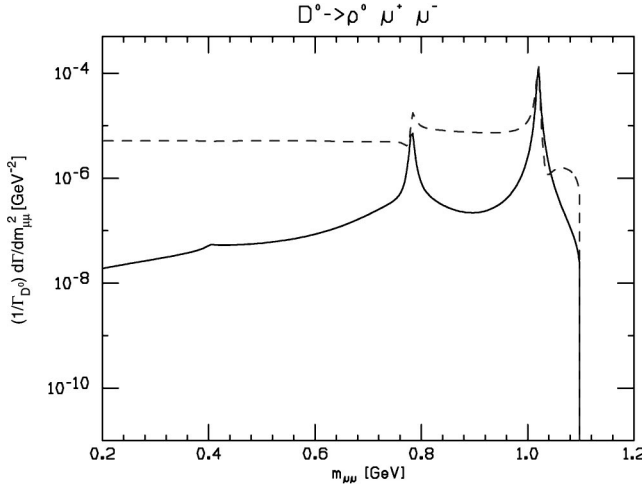
FIG. 13. The dilepton mass distribution for D^0 \rightarrow \rho^0 \mu^+ \mu^- normalized to \Gamma_{D^0} . The solid line shows the sum of the short and the long distance SM contributions. The dashed line includes the allowed R -parity violating contribution from supersymmetry (see text for details).
