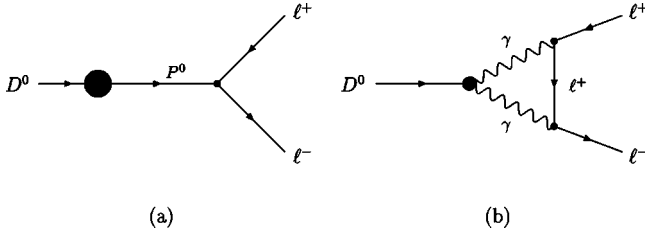
FIG. 8. Unitarity contributions: (a) One-particle. (b) Two-particle \gamma\gamma .
