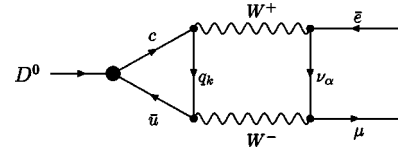
FIG. 15. Box diagram mediating D^0 \rightarrow \mu \bar{e} .
