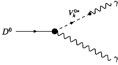
FIG. 5. Vector dominance (VMD) contribution.
