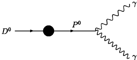
FIG. 6. Weak mixing contribution.
