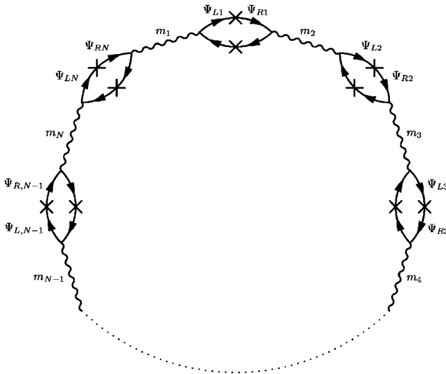
FIG. 3. Graphical depiction of the Hamiltonian \mathcal{H}_N in Eq. (5). Fermions transform as indicated in Eq. (1) under the weak gauge groups SU(m)_k , whose bosons are identified in the figure. An \times indicates a dynamical mass insertion. Strong SU(n) gauge boson interactions within each fermion loop are not indicated. There are no strong gauge interactions between loops.
