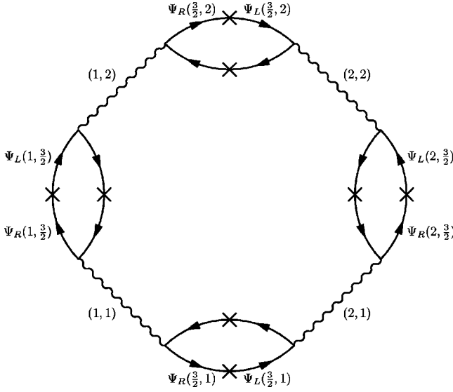
FIG. 8. Typical graph contributing to the Hamiltonian \mathcal{H}_4 in Eq. (29). The notation is as in Fig. 7.
