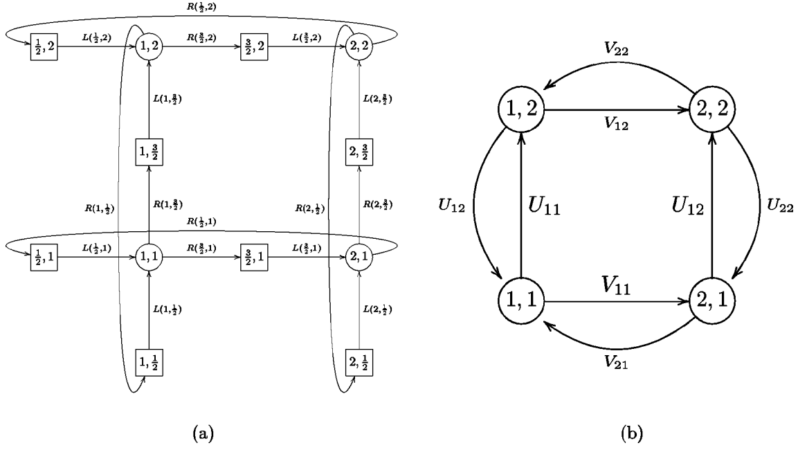
FIG. 6. The full (a) and condensed (b) moose for the N=2 toroidal model of Ref. [2] with a QCD-like UV completion. Notation is as in Figs. 4 and 5.
