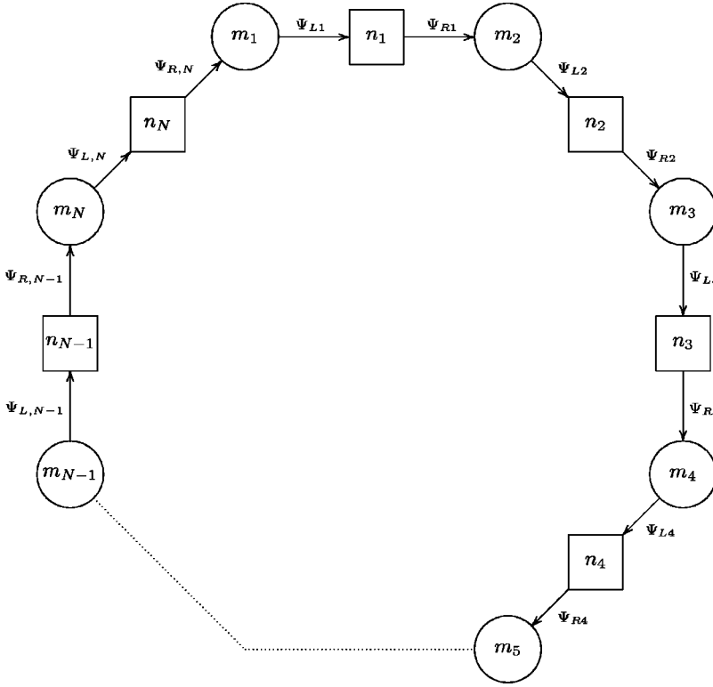
FIG. 1. The full moose for the ring model of Ref. [1], showing its UV completion. Strong gauge groups are labeled by n_1, n_2, \dots, n_N and weak gauge groups by m_1, m_2, \dots, m_N . Fermions \psi_{Lk} and \psi_{Rk} transform as (n, m, 1) and (n, 1, m) of (\text{SU}(n)_k \otimes \text{SU}(m)_k \otimes \text{SU}(m)_{k+1}) .
