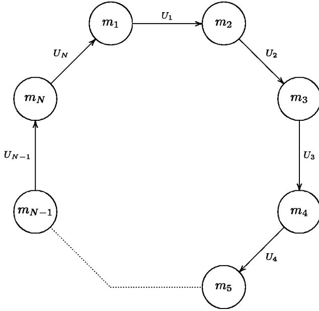
FIG. 2. The condensed moose for the ring model of Ref. [1], characterizing its low-energy structure with nonlinear sigma fields U_k = \exp(i\pi_k/f) linking the weak groups SU(m)_k and SU(m)_{k+1} .
