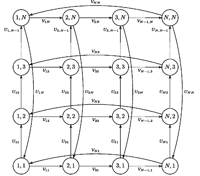
FIG. 4. The condensed moose for the toroidal model of Ref. [2]. The weak SU(m)_{kl} group is denoted by a circle at the site (k, l) . The site (k, l) is identified with the sites (k+N, l) and (k, l+N) . Nonlinear sigma model link fields U_{kl} and V_{kl} transform according to Eq. (7).
