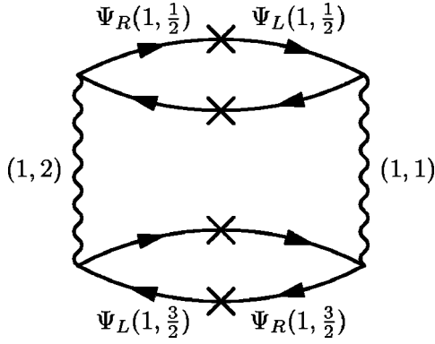
FIG. 7. Graphical depiction of a typical term in the Hamiltonian \mathcal{H}_2 in Eq. (23). Fermions transform as indicated in Fig. 6(a) under the weak gauge groups SU(m)_{kl} , whose bosons are identified in the figure. An \times indicates a dynamical mass insertion. As in Fig. 3, strong SU(n) gauge boson interactions within each fermion loop are not indicated and there are no strong gauge interactions between loops.
