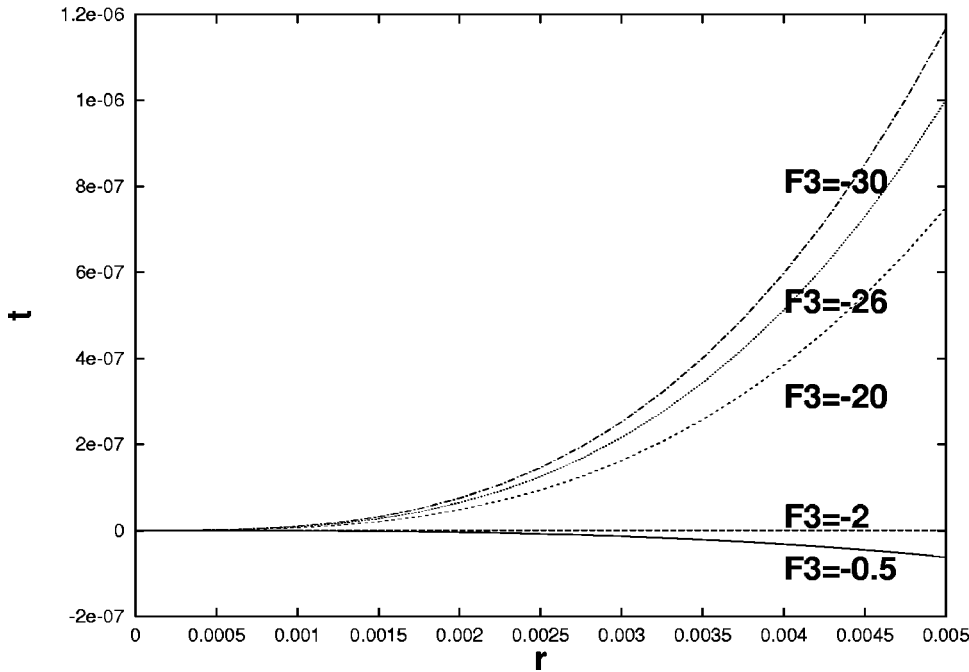
FIG. 1. Apparent horizon curves near r=0 for the n=3 case, with F_0=1 . The labels on the curves give the values of F_3 , the nonvanishing coefficient quantifying the shear. A black hole forms if F_3 \geq -2 .
