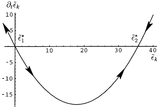
FIG. 1. Fixed-point structure of the \tilde{\epsilon}_k flow equation after fermion-boson translation by hand. The graph is plotted for the threshold functions discussed in Appendix E with e = 1 . Note that \tilde{\epsilon}_1^* is small but different from zero [cf. Eq. (22)]. Arrows indicate the flow towards the infrared, k \rightarrow 0 .
