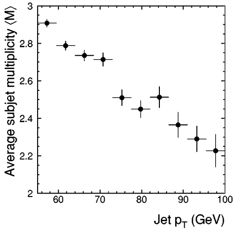
FIG. 19. Uncorrected mean subjet multiplicity versus jet p_T in D\bar{D} data at \sqrt{s} = 1800 GeV. Note the suppressed zero on the vertical axis.
