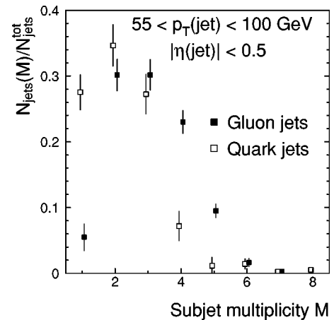
FIG. 22. Uncorrected subjet multiplicity in gluon and quark jets, extracted from D\bar{D} data at \sqrt{s} = 1800 GeV and 630 GeV, using nominal gluon-jet fractions f_{1800} = 0.59 and f_{630} = 0.33 .
