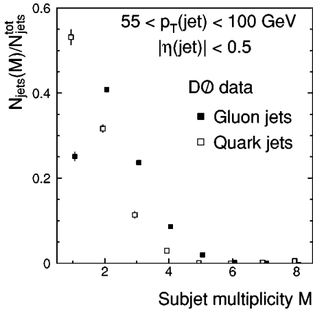
FIG. 29. Corrected subjet multiplicity for gluon and quark jets, extracted from D0 data.
