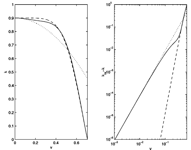
FIG. 5. Comparing our full ansatz for the momentum parameter (3.9) (solid line), and the simpler expressions for the relativistic and friction dominated regimes, Eqs. (3.10) and (3.11) (dashed and dotted, respectively), for relativistic (left panel) and non-relativistic (right panel) velocities.
