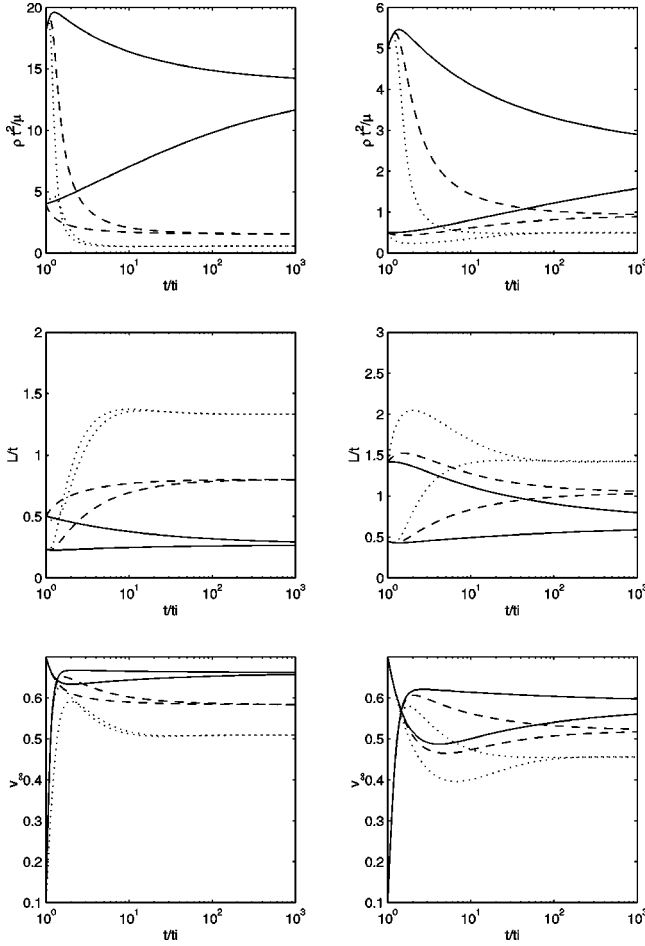
FIG. 6. The effect of gravitational back reaction on the approach to scaling of a GUT-scale cosmic string network. Left-side panels correspond to the radiation era, while right-side ones are for the matter era. All plots have \tilde{c}=0.23 ; the back reaction parameter is respectively \Sigma=0 (solid curves), \Sigma=1.25 (dashed) and \Sigma=5.5 (dotted). For each case two curves are plotted, corresponding to initial conditions typical of a first-order (low density and velocity) or second-order (high density and velocity) phase transition. The effect of friction due to particle scattering has been neglected, in order to mimic currently existing numerical simulations.
