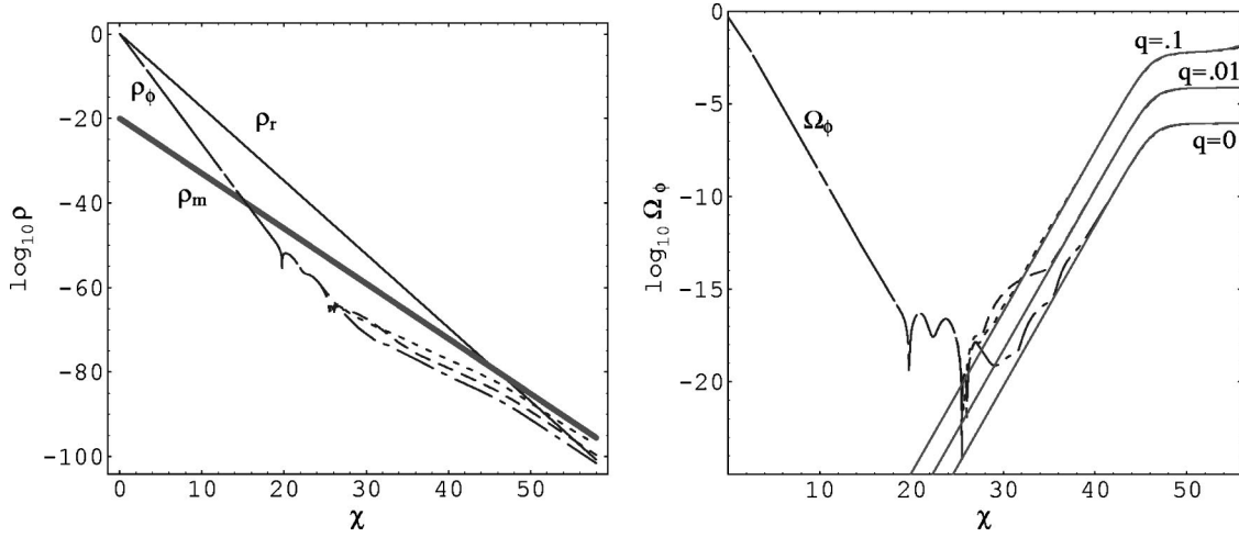
FIG. 2. Time evolution of \rho_\phi for q=0 (dash-dotted curve), q=0.01 (dashed curve) and q=0.1 (dotted curve). The initial scale is a_i = 10^{-20} a_{\text{eq}} , and the epoch of matter-radiation equality corresponds to \chi \approx 46 . Left panel: the dilaton energy density is compared with the radiation (thin solid curve) and matter (bold solid curve) energy density. Right panel: the dilaton energy density (in critical units) is compared with the analytical estimates (4.12), (4.13), (4.14) for the focusing and dragging phases.
