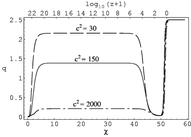
FIG. 5. Time evolution of q(\phi) , from Eq. (5.4), for three different values of the parameter c . All the other parameters are the same as in the example of Fig. 3. During the dragging phase the value of q converges to the regime q \ll 1 .
