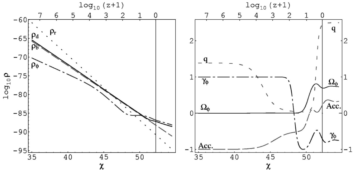
FIG. 3. Left panel: Late-time evolution of the dark matter (solid curve), barionic matter (dashed curve), radiation (dotted curve) and the dilaton (dash-dotted curve) energy densities, for the string cosmology model specified by Eqs. (5.4),(5.5). The upper horizontal axis gives the \log_{10} of the redshift parameter. Right panel: for the same model, the late-time evolution of q (fine-dashed curve), w_\phi (dash-dotted curve), \Omega_\phi (solid curve) and of the acceleration parameter \ddot{a}/\dot{a}^2 (dashed curve).
