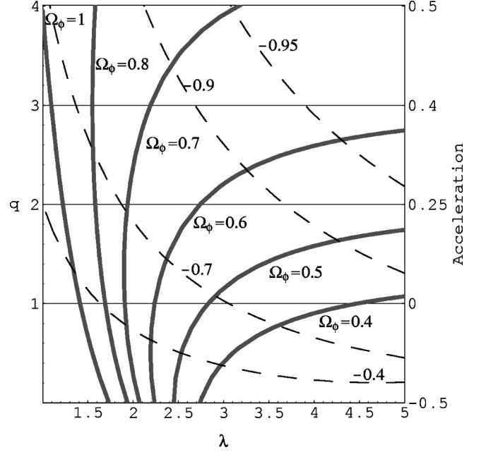
FIG. 1. The asymptotic configurations in the plane \{\lambda, q\} . The full bold curves correspond to asymptotic solutions with fixed ratios \rho_\phi/\rho_d and with the following values of \Omega_\phi : 1, 0.8, 0.7, 0.6, 0.5, 0.4. On the right vertical axis we have reported the corresponding q -dependent acceleration parameter, \ddot{a}a/\dot{a}^2 . The thin dashed curves correspond to fixed asymptotic values of the dilaton equation of state w_\phi = p_\phi/\rho_\phi , respectively -0.4 , -0.7 , -0.9 and -0.95 .
