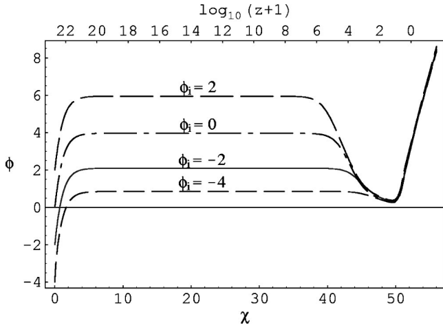
FIG. 4. Time evolution of the dilaton field, for different initial conditions \phi_i = -4, -2, 0, 2 . All the other parameters are the same as in the example of Fig. 3. After the plateau associated with the focusing regime, and for a strong enough dilaton charge, the solutions tend to converge to a common value of \phi . The subsequent running to +\infty , driven by the potential, is thus completely independent of the initial value.
