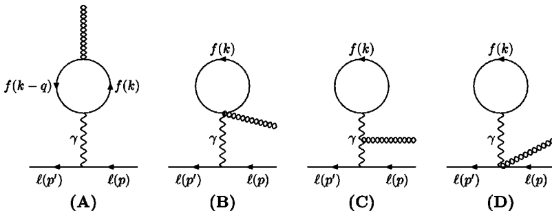
FIG. 3. Diagrams for the one-loop contribution to the gravitational vertex of any charged lepton in a background of electrons and nucleons.
