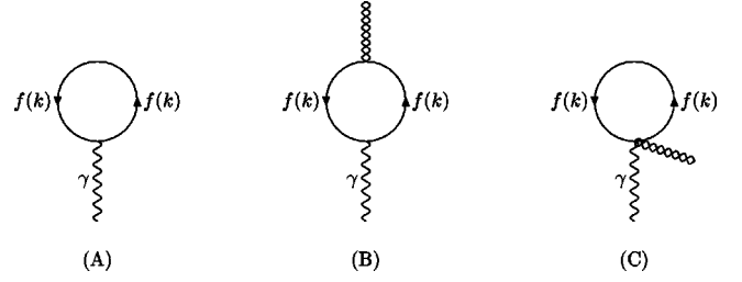
FIG. 4. One-loop diagrams contributing to the photon tadpole in a medium in the presence of a gravitational field. The fermion loop involves a sum over all species of fermions present in the medium.
