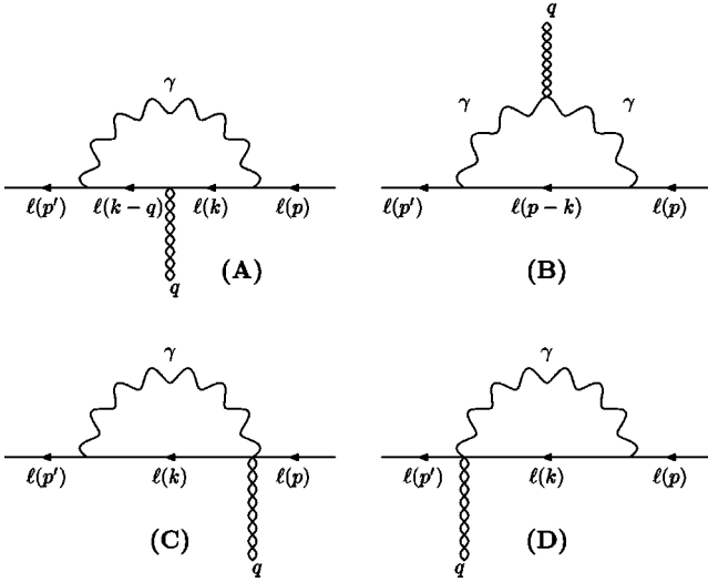
FIG. 2. One-loop diagrams for the gravitational vertex of charged leptons in a background of electrons. The braided line represents the graviton.
