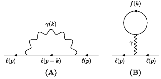
FIG. 1. One-loop diagrams for the self-energy of a charged lepton l in a medium.
