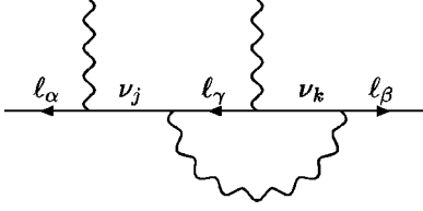
FIG. 3. A higher order correction to diagram (b) of Fig. 1.
