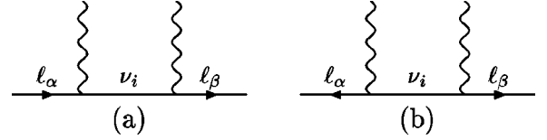
FIG. 1. The two basic subdiagrams for processes that do not involve neutrinos in the external states. Diagram (a) conserves total lepton number, while diagram (b) changes it by two units.
