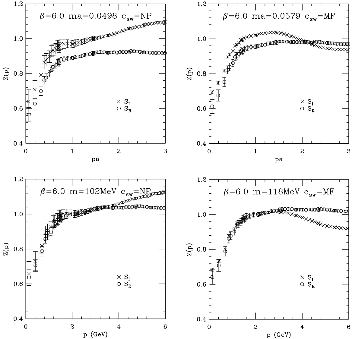
FIG. 4. The tree-level corrected Z(p) , for c_{sw}=\text{NP}, \kappa=0.137 (left) and c_{sw}=\text{MF}, \kappa=0.13344 (right). The upper two figures show the data in lattice units, and without rescaling. The lower two figures show Z(p) vs momentum in physical units, and after rescaling (“renormalizing”) so that Z(2.1 \text{ GeV})=1 . The infrared agreement after rescaling is very good and we take the tree-level corrected Z(p) from S_R with the nonperturbative c_{sw} as the best estimate for this quantity (see text).
