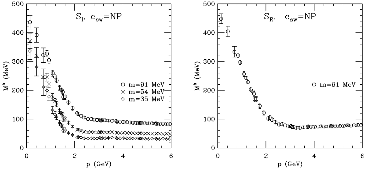
FIG. 6. The hybrid tree-level corrected M^h(p) , for c_{sw} = NP , using S_I (left) and S_R (right). For \tilde{m} = 91 MeV we find good agreement between the two data sets, both in the infrared and ultraviolet. The residual disagreement at intermediate momenta is a pointer to lattice artifacts that we have not brought under full control, even with nonperturbative improvement and hybrid tree-level correction.
