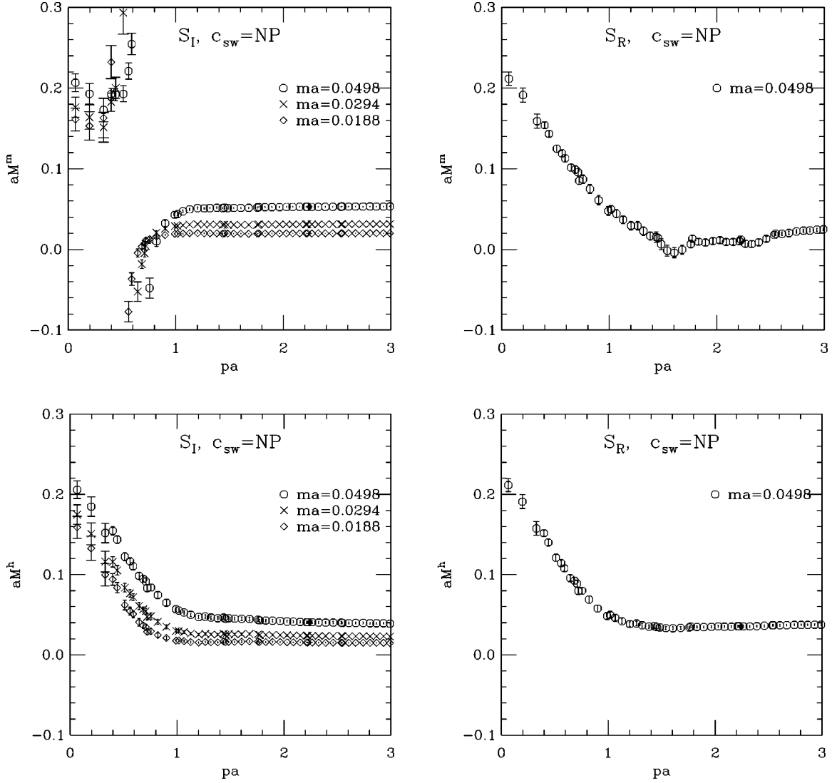
FIG. 5. The tree-level corrected M(p) , for c_{sw} = \text{NP} , using S_I (left) and S_R (right), and with the multiplicative (top) and hybrid (bottom) correction schemes. The multiplicative scheme clearly fails for S_I , and also performs poorly for S_R ; while the hybrid scheme performs well for both and leads to good agreement between the two propagators.
