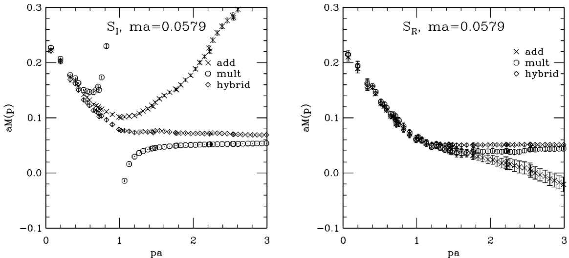
FIG. 1. The tree-level corrected mass function, for S_I (left) and S_R (right) with c_{\text{sw}}=\text{MF}, \kappa=0.13700 , using additive, multiplicative and hybrid correction. The hybrid scheme is robust even in the presence of a zero crossing of the tree-level mass function for S_I .
