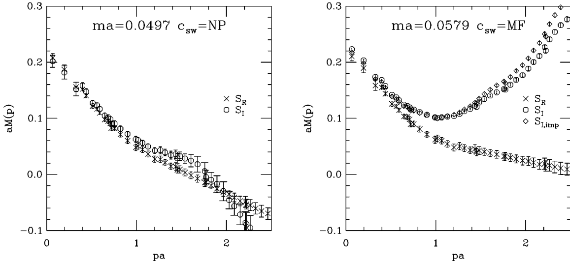
FIG. 2. The additively tree-level corrected mass function, for c_{sw} = \text{NP}, \kappa = 0.13344 (left) and c_{sw} = \text{MF}, \kappa = 0.13700 (right). S_{I,\text{imp}} in the right-hand figure is obtained using the mean-field improved rather than the tree-level values for b_q and \lambda in Eq. (2).
