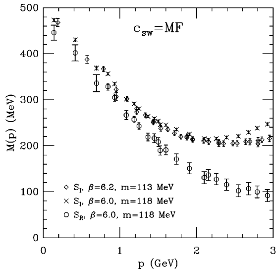
FIG. 3. The additively tree-level corrected mass function, for c_{sw} = \text{MF} , at \beta = 6.2 and \beta = 6.0 .
