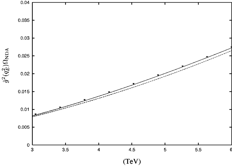
FIG. 7. Graphs of the dimensionless gauge couplings. The solid line and the dashed line represent the effective coupling of Eq. (C7) and Eq. (7.11), respectively. We also plot with the white triangles the coupling directly calculated from the definition of Eq. (7.7) without using approximation Eq. (C5). In this graph, we took C_G=3 , N_f=0 , R^{-1}=3 TeV, \Lambda=6 TeV.
