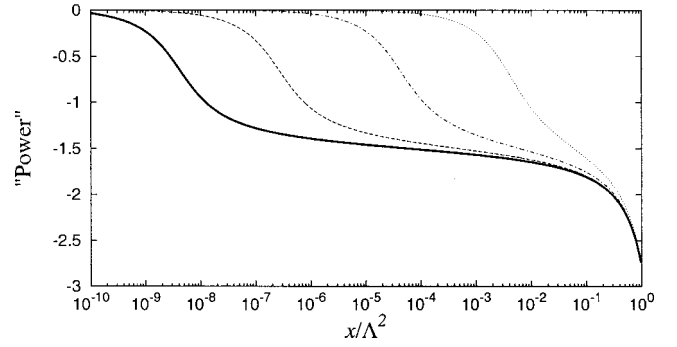
FIG. 5. The “power” behavior of the mass function in eight dimensions. The lines from left to right represent graphs for \kappa_8 = 0.146, 0.147, 0.150, 0.160 [or B^2(M_0^2)/\Lambda^2 = 5.8 \times 10^{-9}, 4.1 \times 10^{-7}, 6.8 \times 10^{-5}, 6.8 \times 10^{-3} ] with \Lambda^2/M_0^2 = 10^{10} .
