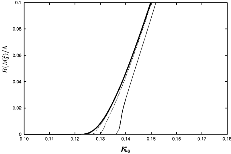
FIG. 2. The scaling behavior in six dimensions. The lines from right to left are graphs for \Lambda^2/M_0^2=10^3,10^4,10^5,10^6,10^{10} , respectively.
