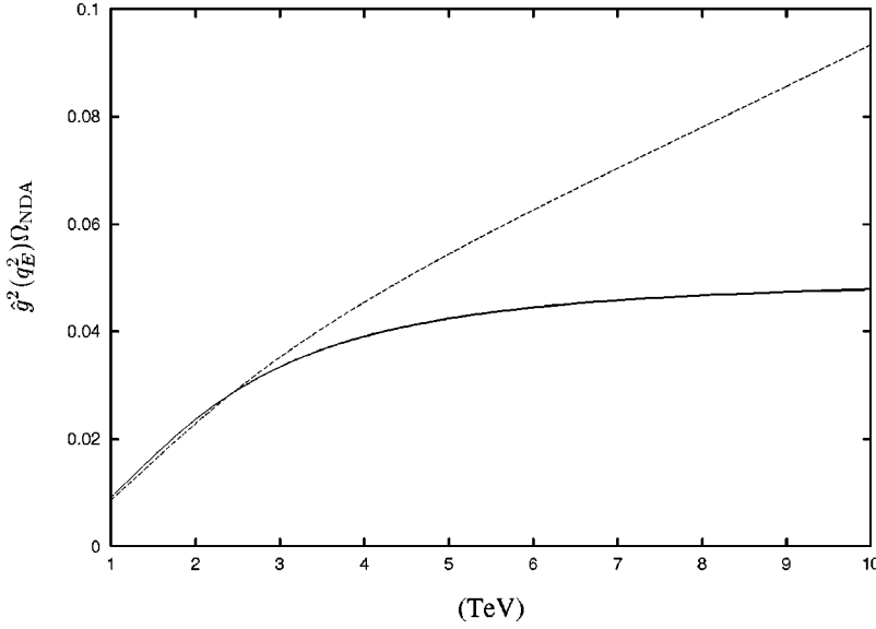
FIG. 6. The graph of the dimensionless gauge coupling with C_G=3 , N_f=0 , R^{-1}=1 TeV, \Lambda=10 TeV, \alpha_{\overline{\text{MS}}}(M_Z)=0.1 . The solid line and the dashed line represent the \overline{\text{MS}} coupling and the effective coupling of Eq. (7.11), respectively.
