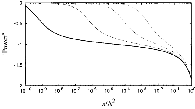
FIG. 4. The “power” behavior of the mass function in six dimensions. The lines from left to right represent graphs for \kappa_6 = 0.122, 0.125, 0.130, 0.140 [or B^2(M_0^2)/\Lambda^2 = 4.1 \times 10^{-10}, 5.4 \times 10^{-7}, 6.9 \times 10^{-5}, 2.2 \times 10^{-3} ] with \Lambda^2/M_0^2 = 10^{10} .
