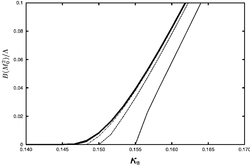
FIG. 3. The scaling behavior in eight dimensions. The lines from right to left are graphs for \Lambda^2/M_0^2=10^3,10^4,10^5,10^6,10^{10} , respectively.
