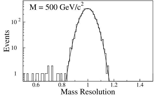
FIG. 83. The distribution of M^{\text{smear}}/M^{\text{unsmear}} for PYTHIA-generated events with |\eta^{\text{jet}}| < 1.0 and 490 < M^{\text{unsmear}} < 510 \text{ GeV}/c^2 .
