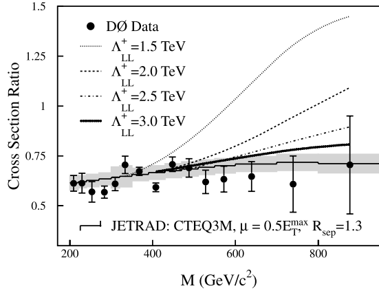
FIG. 97. The ratio of cross sections for |\eta^{\text{jel}}| < 0.5 and 0.5 < |\eta^{\text{jel}}| < 1.0 for data (solid circles) and theoretical predictions for compositeness models with various values of \Lambda_{LL}^+ (various lines; see Sec. IV B for model details). The error bars show the statistical uncertainties. The shaded region represents the \pm 1\sigma systematic uncertainties about the JETRAD prediction.
