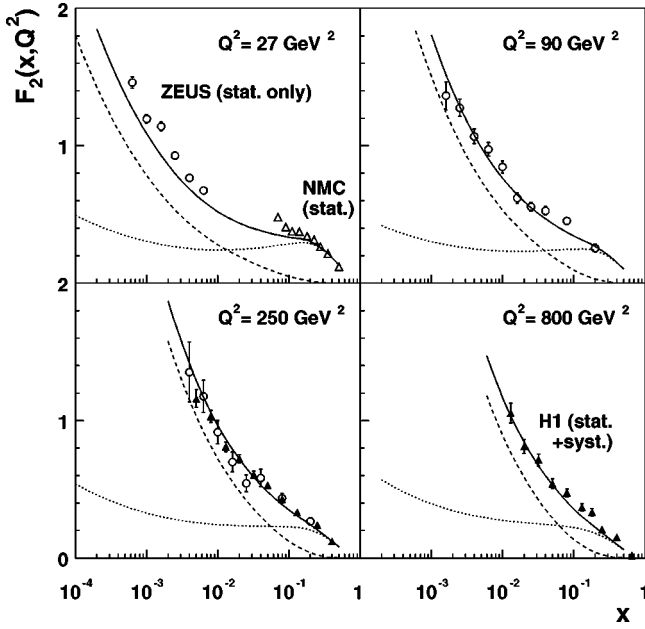
FIG. 5. This is not a fit but the results of using our “DGLAP” unintegrated partons (b) to calculate F_2 ; the gluon-originated contributions are shown as dashed lines and the quark-originated parts are shown as dotted lines. Recent data are plotted [13], and compare well with the sum of the gluon and quark contributions (solid curves), especially at high Q^2 .
