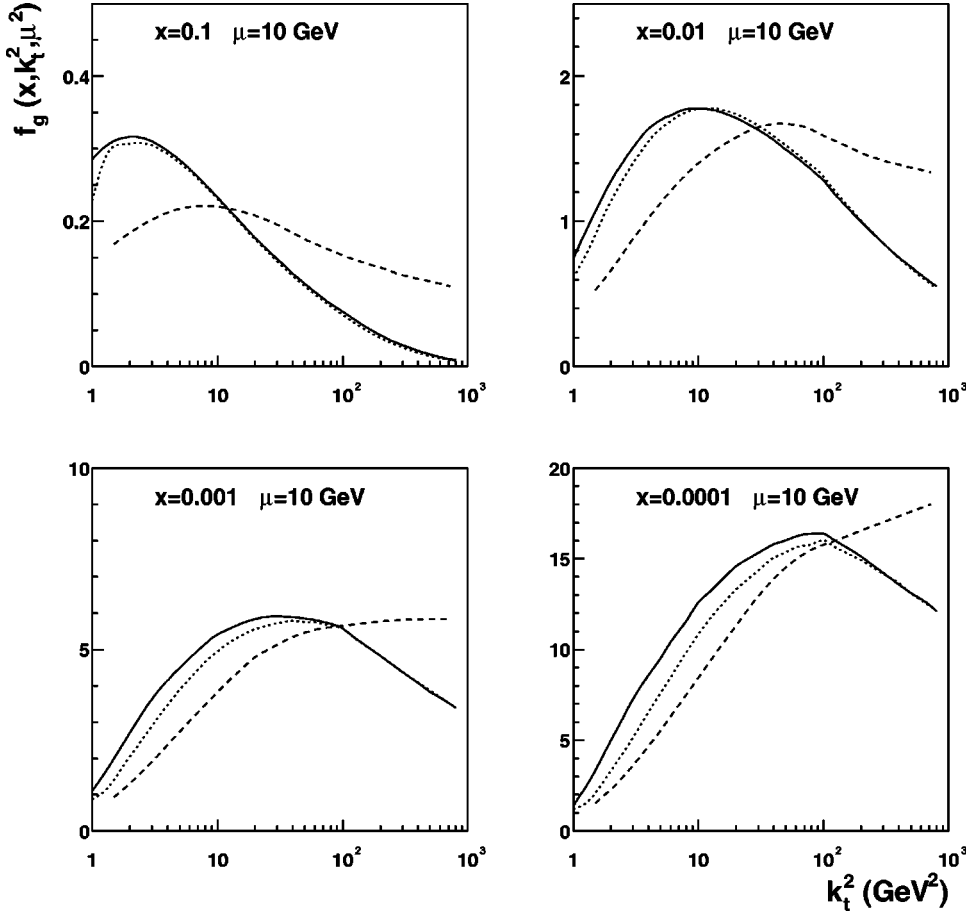
FIG. 3. Plots of the k_t dependence of the unintegrated gluon f_g(x, k_t^2, \mu^2) for various values of x , at \mu = 10 GeV. The solid curves are our version (a) of f_g from Eq. (13); for comparison we show with dashed lines the unintegrated gluon from [5] (as in [5], the dashed lines have been smoothed in the transition region k_t \sim \mu ). Also we plot our “DG-LAP” unintegrated gluon (b) from Eq. (4) in dotted lines, which with the correct angular ordering cutoff is very close to the new f_g , especially at high x .
