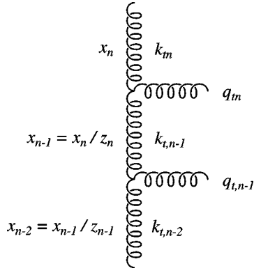
FIG. 2. Part of the evolution chain. We commonly write k_t for k_m and then the parent's transverse momentum as k_t' . The radiated transverse momentum is q_t . Unified evolution is naturally performed [5] in terms of the rescaled transverse momentum q_n = q_{tn}/(1 - z_n) .
