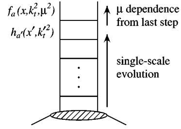
FIG. 1. An illustration of our procedure, in which the evolution of a single-scale unintegrated parton is followed by a final step of the ladder which introduces dependence on the second hard scale, \mu .
