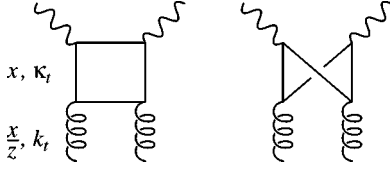
FIG. 4. The quark box, and crossed-box, diagrams which mediate the contribution of the unintegrated gluon distribution f_g(x/z, k_t^2, \mu^2) to F_2 .
