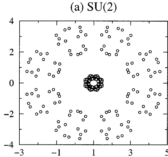
FIG. 6. (a) The spectrum of \Lambda(x) in the complex plane on an 8 \times 8 lattice in SU(2) gauge group.
