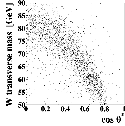
FIG. 5. Smeared W boson transverse mass versus true \cos \theta^* for p_T^W \leq 10 GeV from Monte Carlo simulation. Acceptance cuts have been applied to events in this plot. This correlation plot is used to infer the \cos \theta^* distribution from the measured M_T^W distribution.
