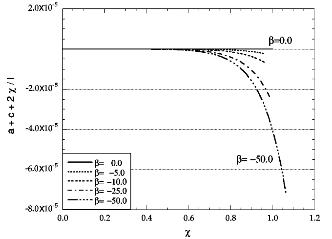
FIG. 3. The quantity a + c + 2\chi/l at r=r_+ plotted for M=5 , Q=0 and \beta=0, -5, -10, -25 and -50 .
