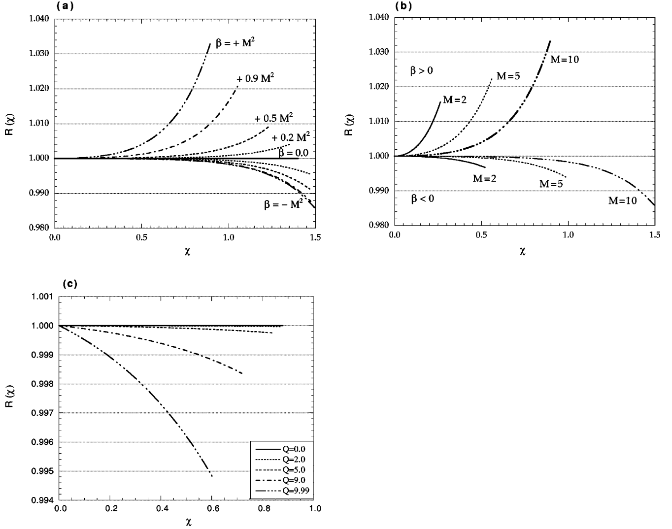
FIG. 1. Ratio of the physical size of apparent horizon to size of black string apparent horizon, R(\chi) [cf. Eq. (3.10)], plotted as a function of \chi . Figure (a) is for model (i). Lines are of \beta=0, \pm 0.2M^2, \pm 0.5M^2, \pm 0.9M^2 and \pm M^2 , where M=10.0 . We see that the qualitative behavior of R(\chi) depends on the sign of \beta . Figure (b) is for the extremal case of model (i), \beta=M^2 with different values of M . Results are also plotted for \beta=-M^2 . Figure (c) is for model (ii) for which R(\chi) is monotonically decreasing.
