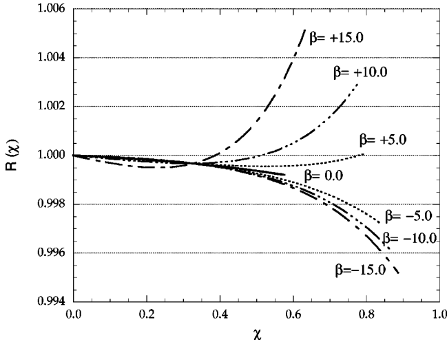
FIG. 2. Ratio of physical size of apparent horizon to size of black string apparent horizon, R(\chi) [cf. Eq. (3.10)], for nonzero Q and \beta . We have set M=5 , Q=3 and \beta=0, \pm 5, \pm 10, \pm 15 for this plot. The main features are a combination of plots in Fig. 1.
