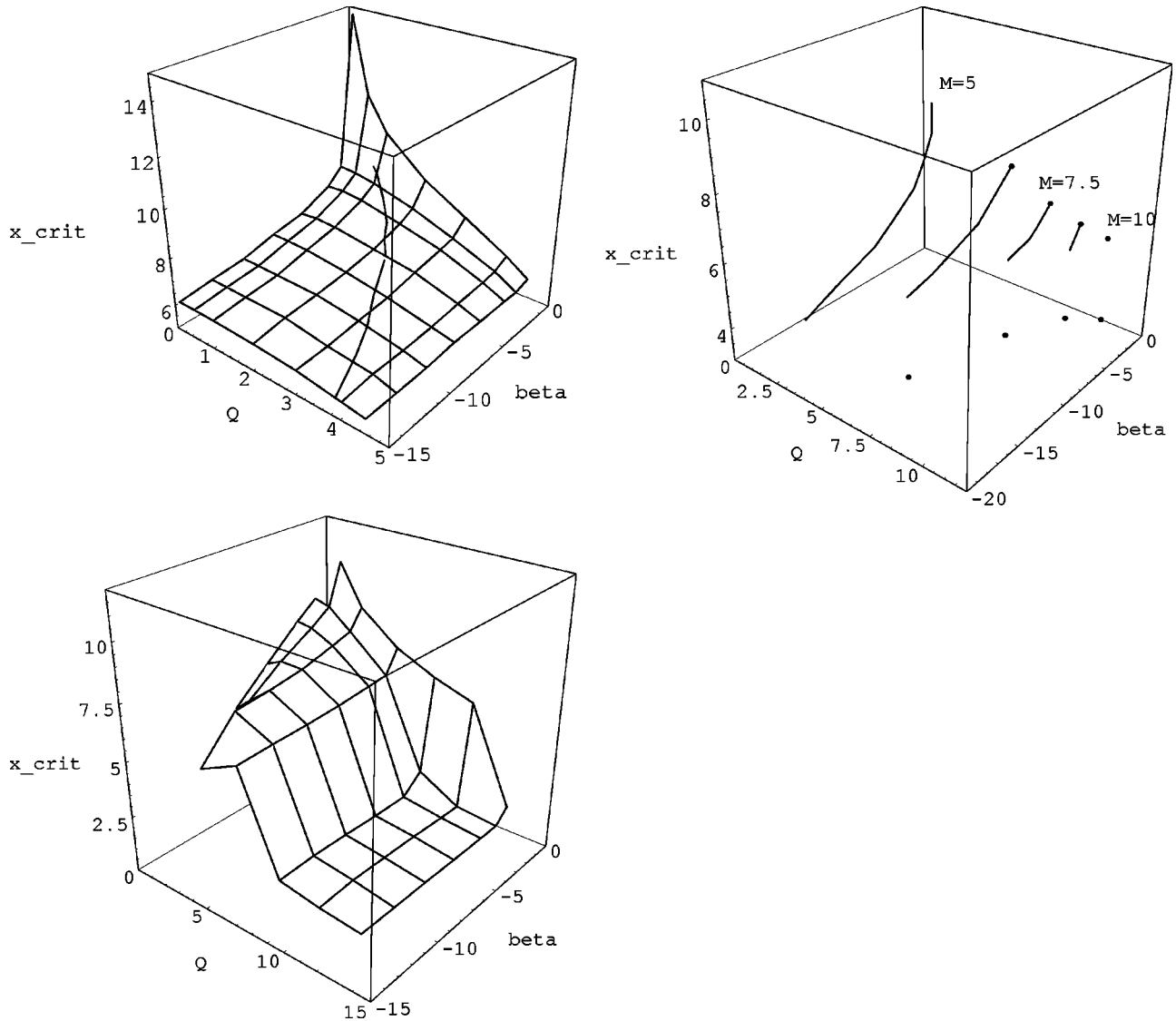
FIG. 4. Critical value \chi_{crit} [Eq. (3.23)] plotted for non-zero Q and \beta(\leq 0) black holes. [above left] We have set M=5 for this plot. Note that for the uncharged case, \chi_{crit}=\infty . The solid curve is for the special cases with r_+=10.0 . [above right] Critical value \chi_{crit} for combinations of parameters (Q,\beta) which produce a black hole with r_+=10.0 . M=5.0,6.25,7.5,8.75 and 10.0 are chosen for these plots. The black dots denote the ends of the lines at \beta=0 and the other ends projected onto the \chi_{crit}=3 plane. [below] The same plot as for (b), but M is specified so as to fix r_+=10 for given (Q,\beta) .
