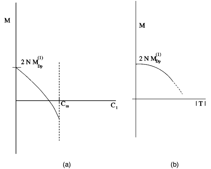
FIG. 3. ADM mass (for a fixed r_0 > 0 ) as a function of (a) c_1 and (b) |T| .
