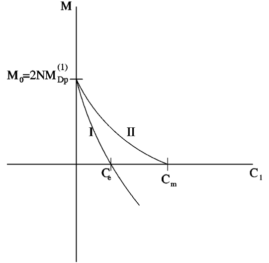
FIG. 2. The two-parameter space of solutions for Q = 0 , as parametrized by M, c_1 . Path II represents decay of the brane-antibrane configuration to flat space.
