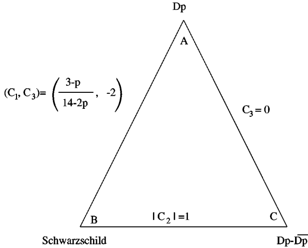
FIG. 5. The most general spherically symmetric solution of type II theories.
