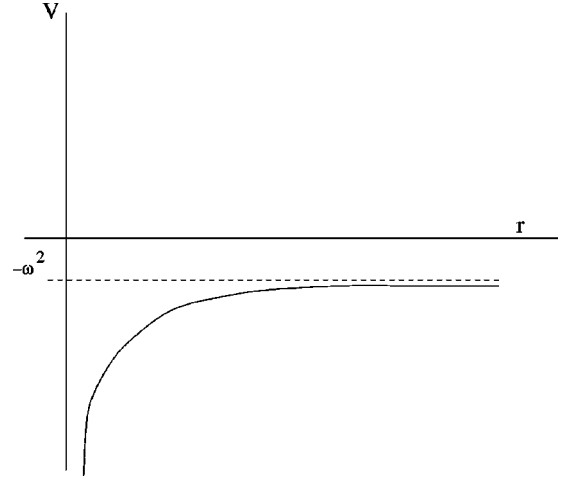
FIG. 4. The scattering potential V(r) for gravitons on Dp - \overline{Dp} -branes.
