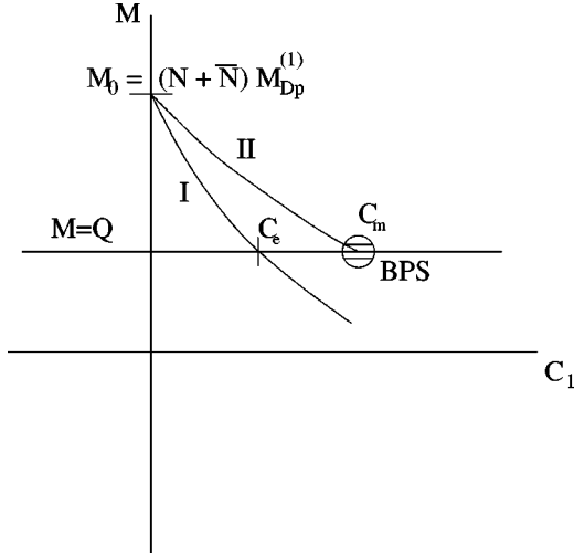
FIG. 1. The M, c_1 plane for a given fixed Q \neq 0 . The BPS solution corresponds to the scaled neighborhood represented by the shaded circle. Path II represents decay to a BPS D-brane of charge Q .
