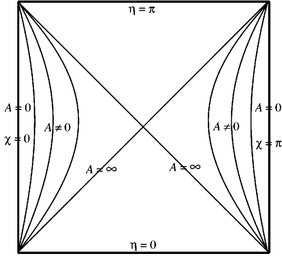
FIG. 1. The conformal diagram for de Sitter space indicating trajectories of observers with uniform acceleration A . Each point represents a complete 2-sphere.
