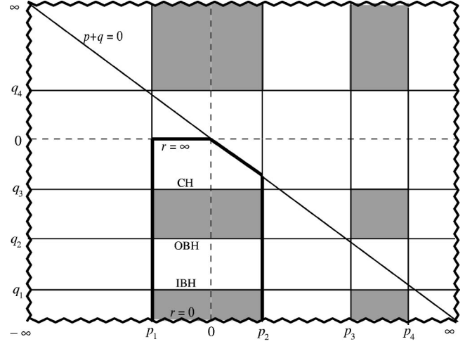
FIG. 3. In the full ranges of p and q , space-times only occur when p lies between the roots p_1 and p_2 , or between p_3 and p_4 . These include six possible static space-time regions which are indicated by the shaded areas. Attention is focused here on the space-time spanned by p_1 < p < p_2 and q < -p . This contains two static and two nonstatic regions separated by a cosmological horizon (CH) and inner and outer black hole horizons (IBH and OBH). Apart from a region near conformal infinity, this space-time is also covered by the coordinates r and \theta which span the regions indicated by the area within the bold lines.
