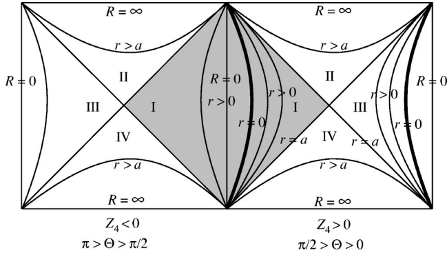
FIG. 2. The conformal diagram for de Sitter space such that each point represents a hemisphere. The shaded area indicates the region I covered by the new coordinates of (10) for 0 \leq r \leq a . The complete space repeats this area in region III and includes the regions II and IV beyond the cosmological horizons. Thus r=0 represents two uniformly accelerating points on causally disconnected opposite sides of the universe.
