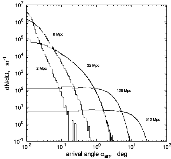
FIG. 5. Angular distribution of the arrival angle at Earth for mono-energetic injection of protons of energy E = 10^{21.5} eV, and for various source distances as indicated. The magnetic field is 1 nG.
