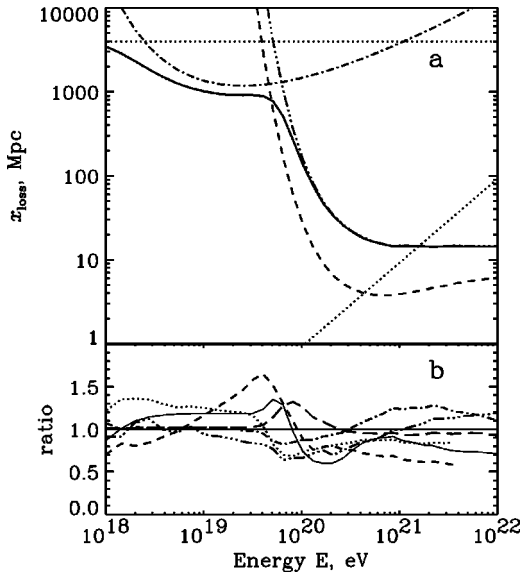
FIG. 1. (a) Mean energy loss length due to adiabatic expansion (upper dotted curve), Bethe-Heitler pair production (dash-dotted curve), and hadron production (triple-dot-dashed curve). Also shown are the hadron interaction length (dashed curve) and the neutron decay length (lower dotted curve). The solid line shows the total x_{\text{loss}} . (b) Ratio of mean energy loss length as calculated in Refs. [8] (dotted), [10] (long-dashed), [9] (short-dashed), [12] (dash-dotted), [13] (dashed-dot-dot-dot), and [25] (thin solid) to the loss length of the present work presented in the upper panel.
