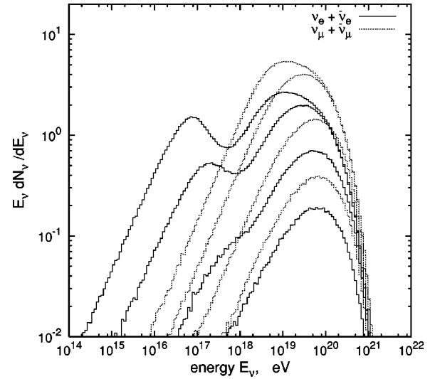
FIG. 6. \nu_\mu + \bar{\nu}_\mu and \nu_e + \bar{\nu}_e spectra at Earth after propagating a mono-energetic proton beam of energy 10^{21.5} eV at distances of 2, 8, 32 and 128 Mpc (from bottom to top) in a 1 nG intergalactic magnetic field.
