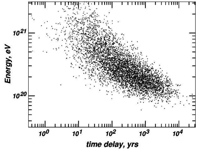
FIG. 4. Scatter plot of time delay versus energy for protons injected with energy of 10^{21.5} eV after propagation over 32 Mpc in random B field of 1 nG.
