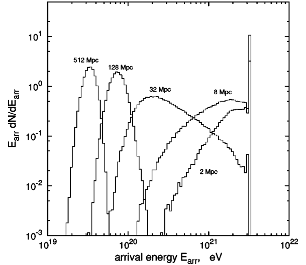
FIG. 2. Arrival spectrum at Earth for mono-energetic injection of protons of energy E = 10^{21.5} eV and for various source distances as indicated. The sharp spike at injection energy for distances D \leq 32 Mpc is due to the low interaction probability within the short distance.
