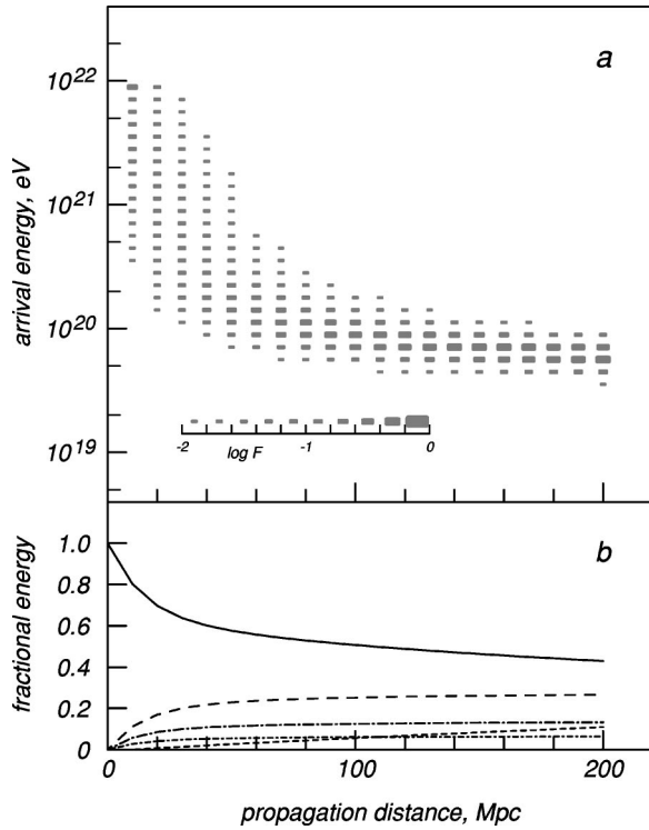
FIG. 8. (a) Arrival energy distribution for protons injected with energy between 10^{21.9} and 10^{22} eV after propagation on 10, 20, ... 200 Mpc. (b) Fractional energy contained in nucleons (solid line), \gamma rays from photoproduction (long dashes) and BH pair production (short dashes) for protons injected with the energy spectrum of Eq. (11). The dash-dot lines show the fractional energy in muon (long) and electron (short) neutrinos and antineutrinos.
