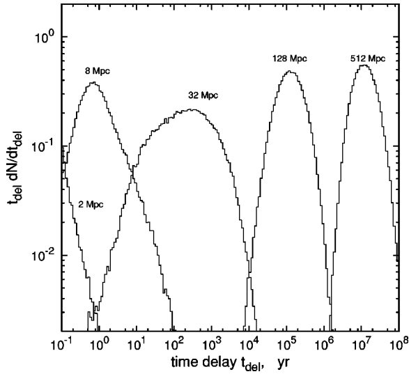
FIG. 3. Time delay of protons injected at different source distances and propagated through a random magnetic field of 1 nG. The time delay is defined as the propagation time of a particle minus the travel time of a light ray along a geodesic.
