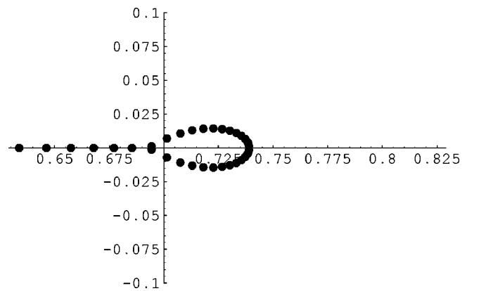
FIG. 1. Solutions of the first 150 coupled Schwinger-Dyson equations for the dimensionless one-point Green's function iG_1 g^{1/3} for the case of a massless zero-dimensional N=3 theory. Note that the solutions (indicated by dots) lie in a small portion of the complex plane very close to the exact answer 0.72901.
