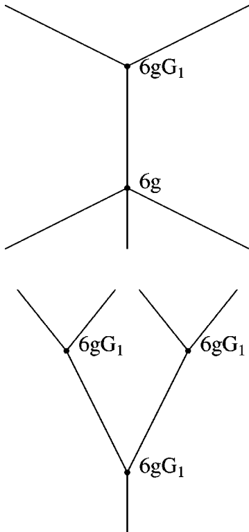
FIG. 5. Lowest order graphs contributing to G_5 .
