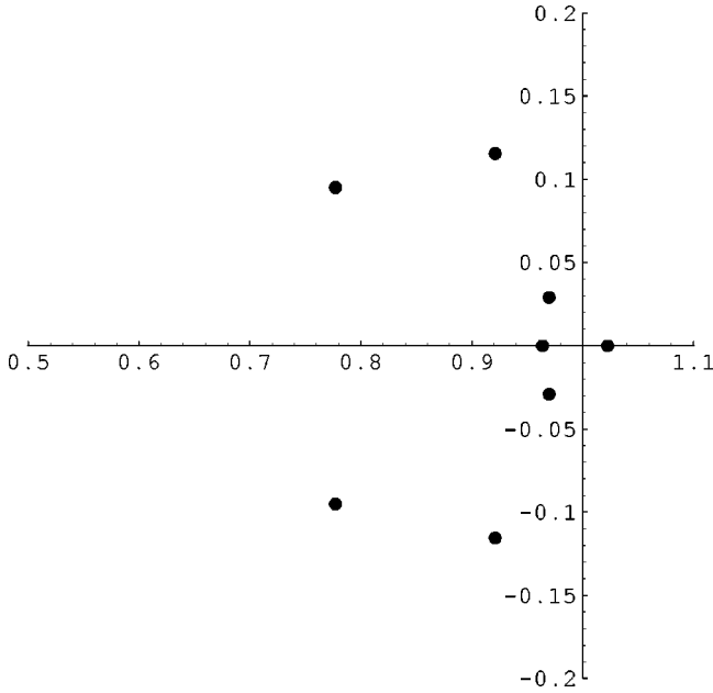
FIG. 2. Solutions of the first ten coupled Schwinger-Dyson equations for the dimensionless one-point Green's function iG_1 g^{1/4} for the case of a massless zero-dimensional N=4 theory. The solutions (indicated by dots) lie in a small portion of the complex plane very close to the exact answer 0.97774.
