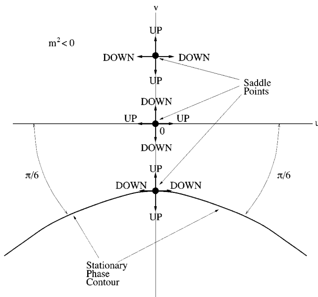
FIG. 4. Saddle points and steepest-descent paths for the function \rho(x) in Eq. (3.9) for the case m^2 < 0 .
