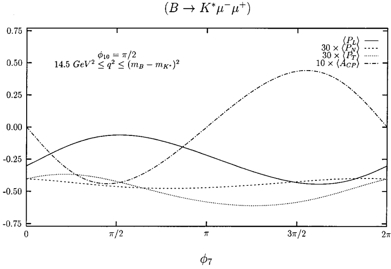
FIG. 4. The same as in Fig. 3 but for \phi_{10} = \pi/2 .
