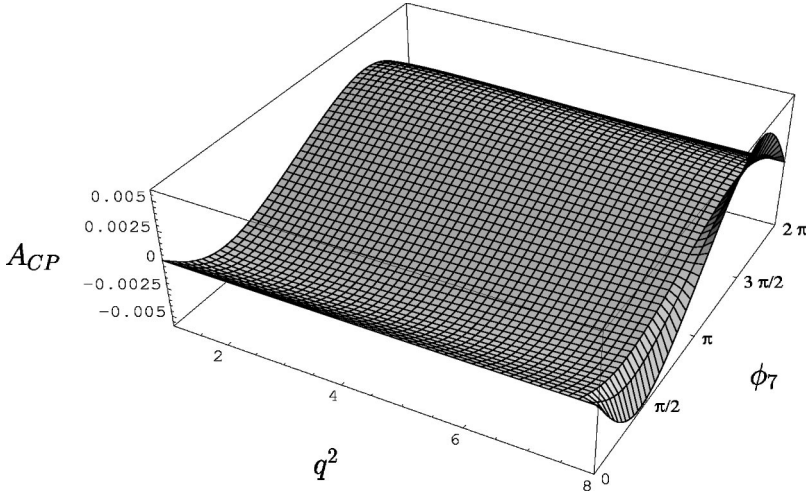
FIG. 1. The dependence of the CP asymmetry A_{CP} for B \rightarrow K^* \mu^- \mu^+ on q^2 and \phi_7 at \phi_{10}=0 for region I.
