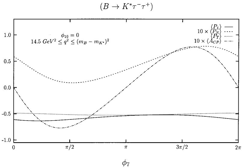
FIG. 5. The same as in Fig. 3 but for B \rightarrow K^* \tau^- \tau^+ decay.
