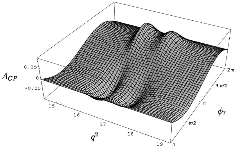
FIG. 2. The same as in Fig. 1 but for region II.
