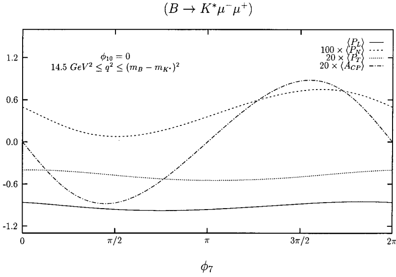
FIG. 3. The dependence of \langle A_{CP} \rangle , \langle P_L \rangle , \langle P_T \rangle , and \langle P_N \rangle for B \rightarrow K^* \mu^- \mu^+ on \phi_7 at \phi_{10} = 0 for region II.
