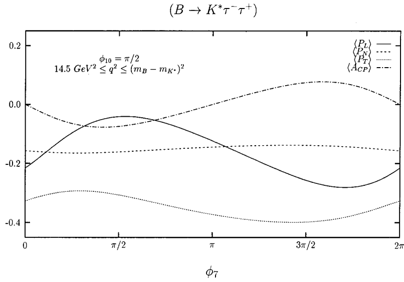
FIG. 6. The same as in Fig. 5 but for \phi_{10} = \pi/2 .
