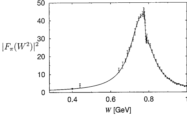
FIG. 10. The square of the electromagnetic pion form factor in the timelike region. The data points are from Ref. [35] and the curve is the parametrization N=1 of Ref. [30].
