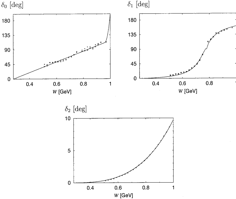
FIG. 6. The phase shifts \delta_0 for the S wave, \delta_1 for the P wave, and \delta_2 for the D wave of elastic \pi\pi scattering. \delta_0 and \delta_2 refer to the I=0 channel. The points are taken from Ref. [28], and the curves for \delta_0 and \delta_2 are simple parametrizations. The curve for \delta_1 corresponds to the parameterization N=1 of the pion form factor F_\pi(W^2) in Ref. [30].
