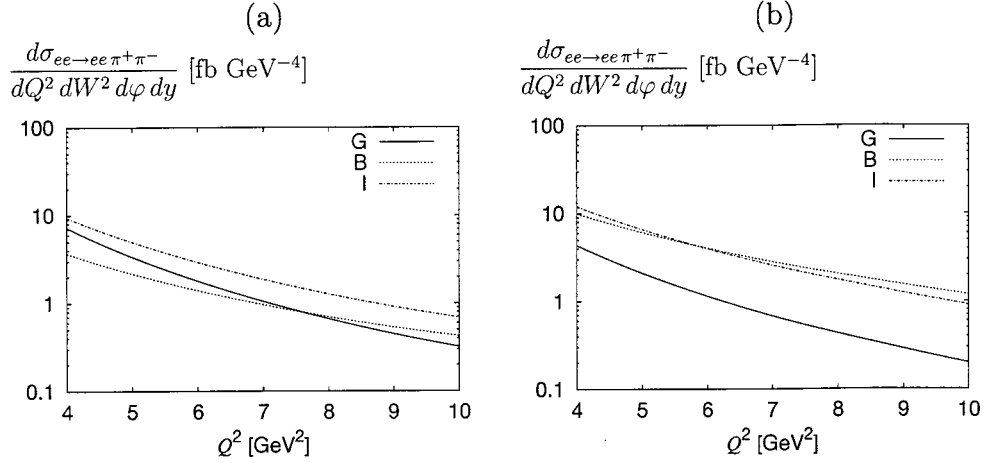
FIG. 11. (a) The contributions to the differential ee cross section from \gamma^*\gamma , bremsstrahlung and their interference. Kinematical variables are W=400 MeV, \varphi=0 , y=0.1 , E_1=3.1 GeV, E_2=9 GeV. For the real photon flux in Eq. (81) we take \alpha_{2L}^{\max}=300 mrad and l_{\perp L}^{\max}=100 MeV as explained in Sec. VIII A. The sign of the interference term corresponds to an e^+\gamma subprocess. (b) The same as (a), but with y=0.2 .
