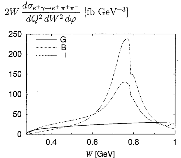
FIG. 13. The W dependence of the different contributions to the differential e^+\gamma cross section at Q^2=5 GeV 2 , \varphi=0 and s_{e\gamma}=50 GeV 2 . The corresponding values of y range from 0.1 to 0.12.
