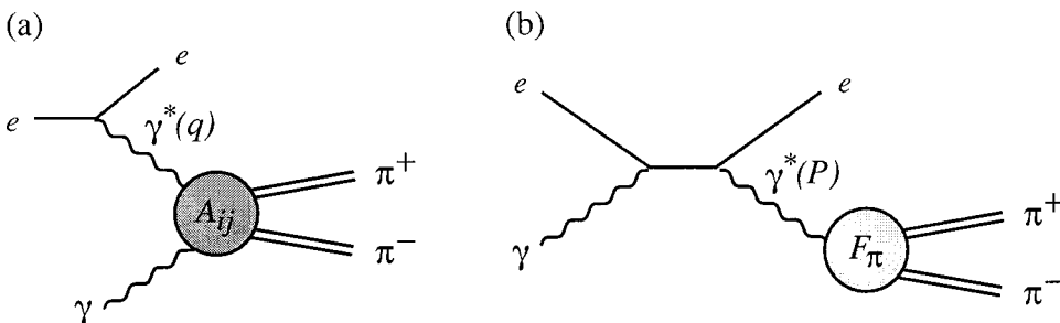
FIG. 9. The two subprocesses contributing to the reaction e\gamma \rightarrow e\pi^+ \pi^- : (a) \gamma^* \gamma scattering and (b) bremsstrahlung. There is a second bremsstrahlung diagram, where the photon vertices are interchanged on the lepton line.
