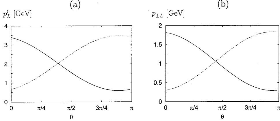
FIG. 18. (a) The pion energies p_L^0 (solid) and p_L'^0 (dotted) in the laboratory as a function of the angle \theta in the two-pion c.m. The values of the remaining kinematical variables are E_1=3.1 GeV, E_2=9 GeV, Q^2=5 GeV 2 , W=400 MeV, y=0.1 , \varphi=0 . (b) The same for the transverse pion momenta p_{\perp L} and p'_{\perp L} in the laboratory.
