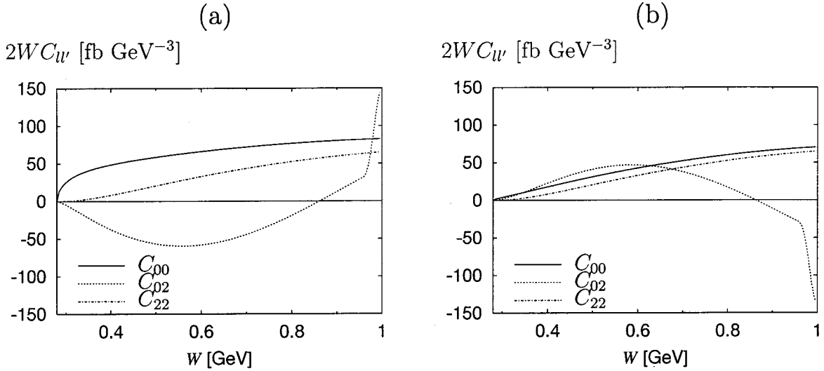
FIG. 8. (a) The coefficients C_{UV} in the differential cross section (87), evaluated with our model GDA (68). They are plotted against W instead of W^2 and therefore have been multiplied with a Jacobian 2W . The values of the remaining kinematical variables are s_{e\gamma} = 50 \text{ GeV}^2 and Q^2 = 5 \text{ GeV}^2 . (b) The same with the alternative ansatz for the GDA described in the text.
