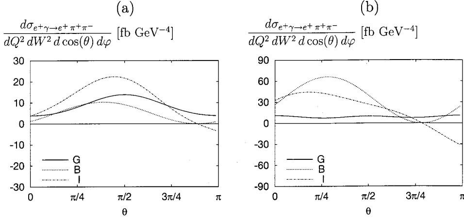
FIG. 15. (a) The \theta dependence of the different contributions to the differential e^+ \gamma cross section at Q^2 = 5 \text{ GeV}^2 , W = 400 \text{ MeV} , \varphi = 0 , and y = 0.1 . (b) The same for W = 800 \text{ MeV} .
