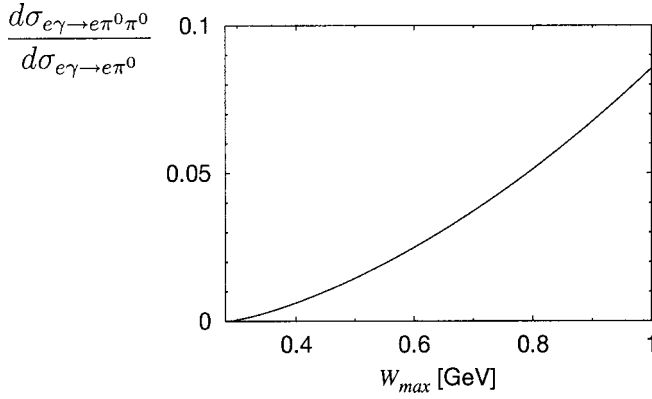
FIG. 7. The ratio of the cross sections (70) and (69) for the production of \pi^0\pi^0 and of \pi^0 in the limit of large Q^2 . The cross section for e\gamma\rightarrow e\pi^0\pi^0 is integrated over W from threshold up to W_{\max} .
