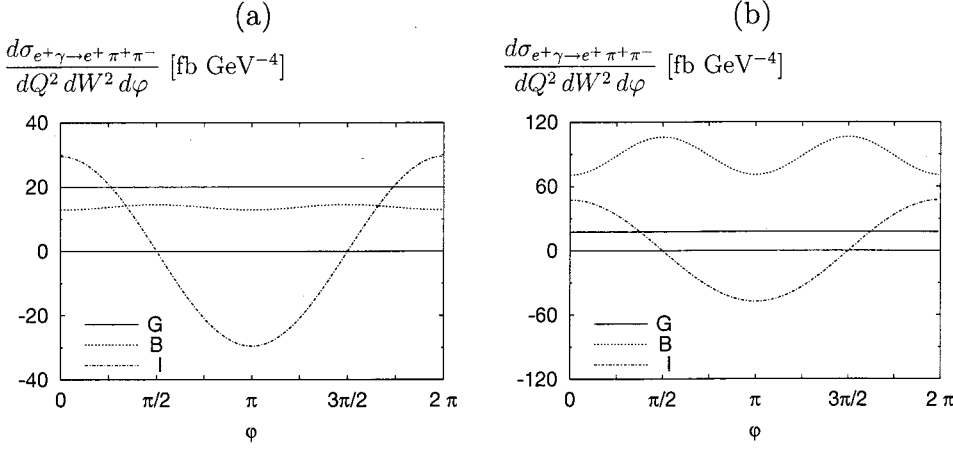
FIG. 14. (a) The \varphi dependence of the different contributions to the differential e^+\gamma cross section at Q^2=5 \text{ GeV}^2 , W=400 \text{ MeV} , and y=0.1 . (b) The same for W=800 \text{ MeV} .
