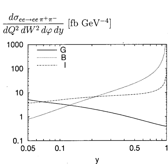
FIG. 12. The same as Fig. 11, but as a function of y at Q^2=5 GeV 2 .
