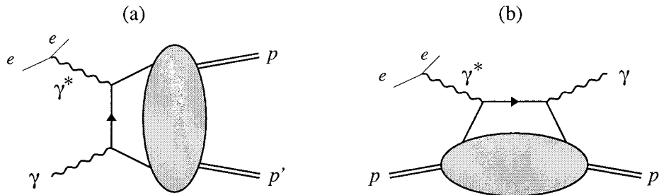
FIG. 3. (a) Factorization of the process \gamma^* \gamma \rightarrow \pi\pi in the region Q^2 \gg W^2, \Lambda^2 . The hard scattering is shown at Born level, with a second diagram being obtained by interchanging the two photon vertices. The blob denotes the two-pion GDA. (b) Crossing relates this process to deep virtual Compton scattering, \gamma^* \pi \rightarrow \gamma\pi . The blob now denotes the (skewed) quark distribution in the pion.
