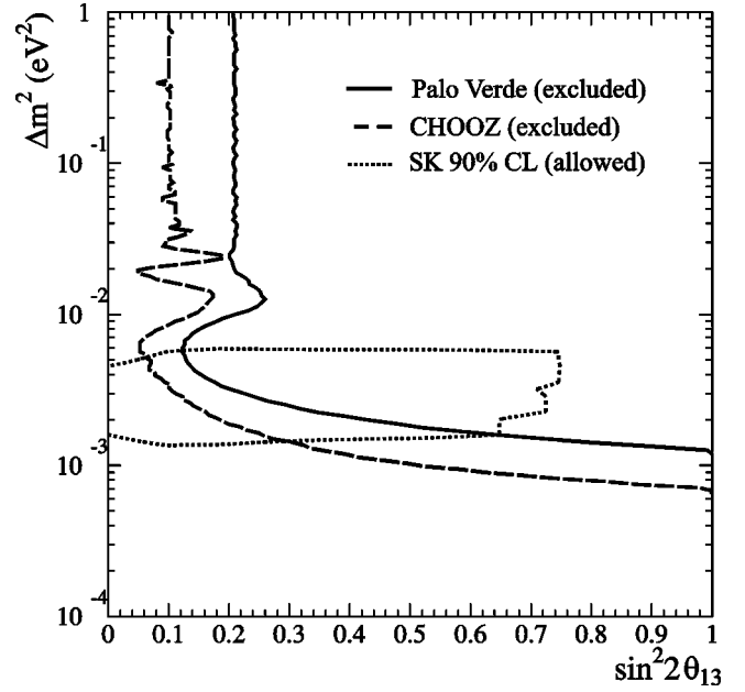
FIG. 24. Exclusion plot showing the allowed region of \theta_{13} and \Delta m^2 based on the Super-Kamiokande preliminary analysis (the region inside the dotted curve). The region excluded by the neutrino reactor experiments are to the right of the corresponding dashed and continuous curves.
