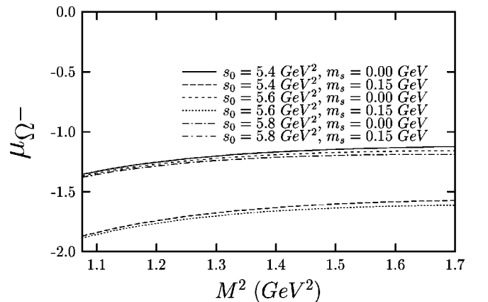
FIG. 6. The same as Fig. 1, but for \Omega^{-} .
