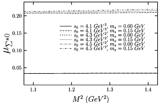
FIG. 2. The same as Fig. 1, but for \Sigma^{*0} .
