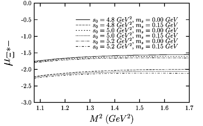
FIG. 5. The same as Fig. 1, but for \Xi^{*-} .
