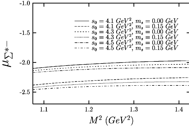
FIG. 3. The same as Fig. 1, but for \Sigma^{*-} .
