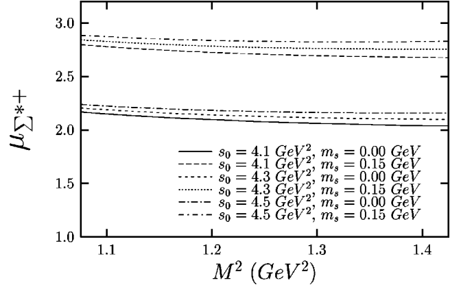
FIG. 1. The dependence of the magnetic moment of \Sigma^{*+} on the Borel parameter, M^2 (in units of nuclear magneton), for three different values of the continuum threshold, s_0 , and for the cases m_s = 0 and m_s = 0.15 \text{ GeV} .
