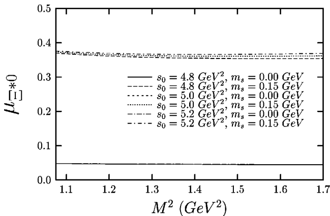
FIG. 4. The same as Fig. 1, but for \Xi^{*0} .
