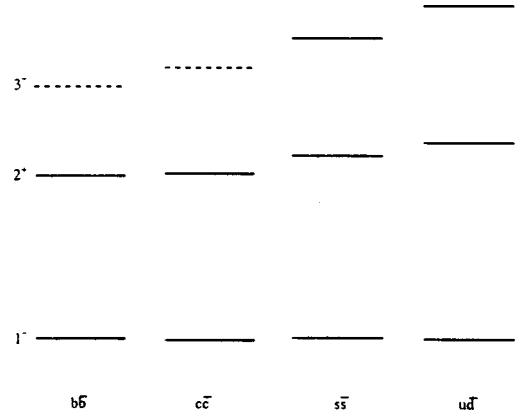
FIG. 2. The orbital excitation spectra of the quarkonia Q\bar{Q} as a function of m_Q ; the 1^- S -waves have been aligned to display the splittings to the P -wave 2^+ and D -wave 3^- states. In b\bar{b} and c\bar{c} , the D -wave positions shown as dashed lines are predictions of reliable heavy quarkonium calculations. The spectra are shown to scale, which may conveniently be calibrated from the \chi_{c2} - \psi splitting of 459 MeV.
