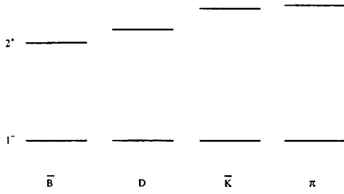
FIG. 3. The orbital excitation spectra of heavy-light mesons as a function of m_Q ; the 1^- S -waves have been aligned to display the splittings to the P -wave 2^+ states. The spectra are shown to scale, which may conveniently be calibrated from the D_2^* - D^* splitting of 452 MeV.
