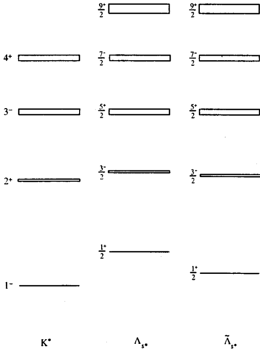
FIG. 4. Comparison of the spectra of well-established ‘‘fully stretched’’ K^* mesons and \Lambda_{s^*} baryons. The boxes show the experimental uncertainties in the masses of states. The l=3 states have been aligned as described in the text. The third spectrum is that of a fictitious \tilde{\Lambda}_{s^*} baryon with the spatial distribution of the ud pair set to zero. The spectra are shown to scale, which may conveniently be calibrated from the K_2^* - K^* splitting of 534 MeV.
