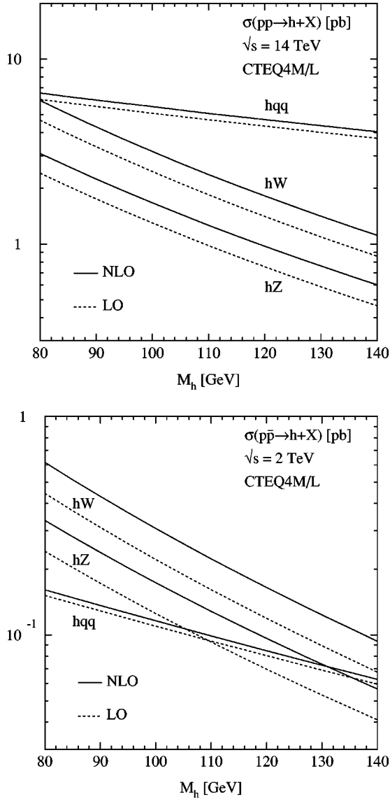
FIG. 2. Total LO and NLO cross sections of Higgs boson production via Higgs-strahlung q\bar{q} \rightarrow h + W/Z and vector boson fusion q\bar{q} \rightarrow q\bar{q} V^* V^* \rightarrow q\bar{q} h [ V=W, Z ] at the LHC (upper plot) and the Tevatron (lower plot) in the decoupling limit.
