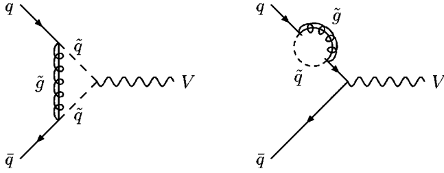
FIG. 1. Generic diagrams contributing to the SUSY-QCD corrections to the q\bar{q}V vertex [ V = \gamma, Z, W ] at NLO.
