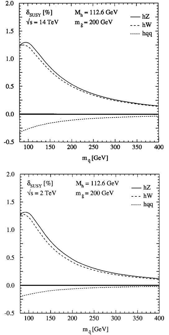
FIG. 3. Relative corrections due to virtual squark and gluino exchange diagrams to Higgs boson production via Higgs-strahlung q\bar{q} \rightarrow h + W/Z and vector boson fusion q\bar{q} \rightarrow q\bar{q} V^* V^* \rightarrow q\bar{q} h [ V=W, Z ] at the LHC (upper plot) and the Tevatron (lower plot).
