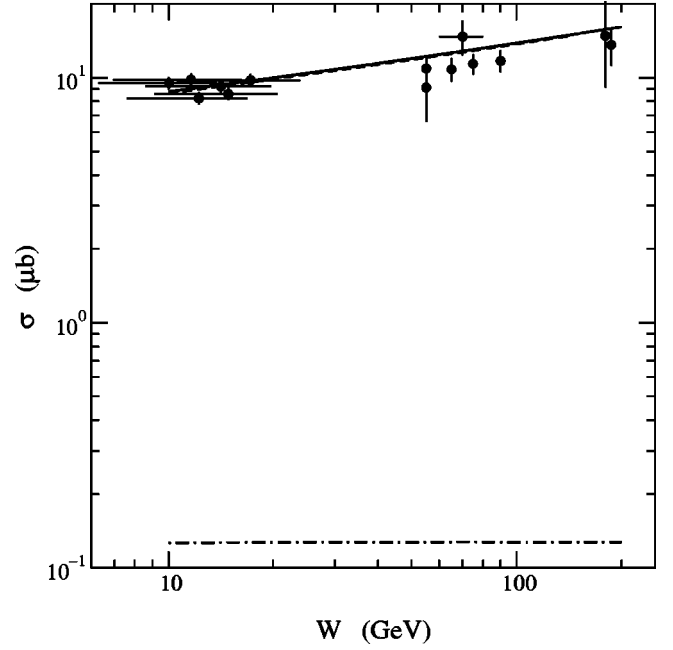
FIG. 3. The cross section for elastic \rho meson photoproduction. The dashed and dot-dashed lines are the contributions from the Pomeron and f_1 exchange, respectively, while the solid line is the total cross section. The experimental data are from Refs. [24,35].
