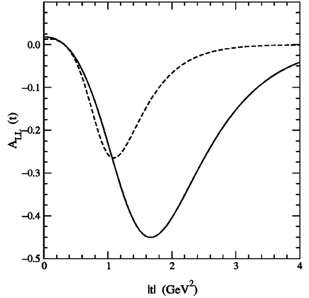
FIG. 7. The double longitudinal asymmetry in elastic proton-proton scattering at \sqrt{s} = 50 GeV (solid line) and at \sqrt{s} = 500 GeV (dashed line).
