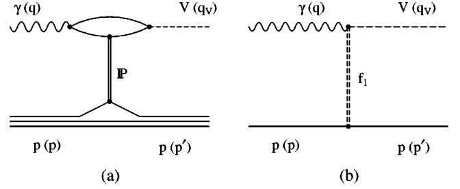
FIG. 2. Vector-meson photoproduction: (a) diffractive process by Pomeron exchange and (b) f_1 exchange.
