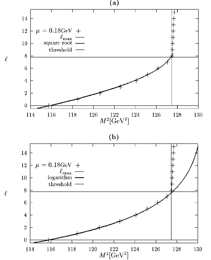
FIG. 1. The parent trajectory for the bottomonium in our model compared to (a) our best fit of the ‘‘square-root’’ form, and (b) our best fit of the ‘‘logarithmic’’ form. The solid vertical line corresponds to the threshold of the quenched lattice potential, i.e., (2M + \sigma/\mu)^2 ; the solid horizontal line shows the maximum l for the data set.
