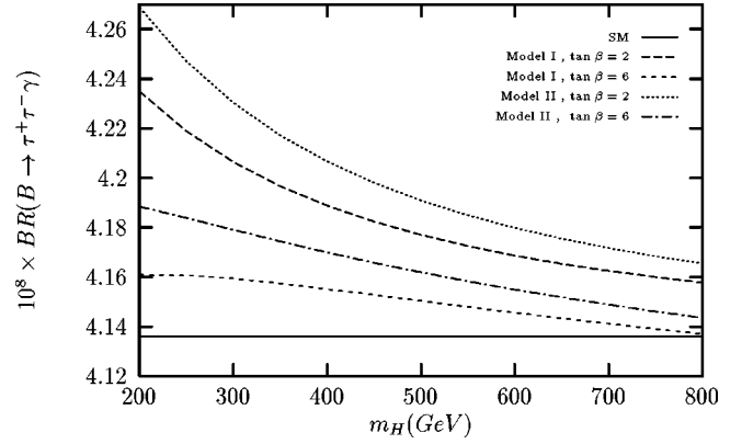
FIG. 2. Branching ratio as a function of m_{H^\pm} in the SM, model I, and II for different values of \tan \beta .
