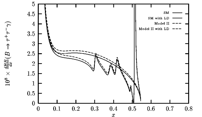
FIG. 1. Differential branching ratio as a function of x = 2E_\gamma/m_{B_s} in the SM and model II for m_{H^\pm} = 400 GeV and \tan \beta = 2 . In this figure, curves with sharp peaks represent the long distance contributions.
