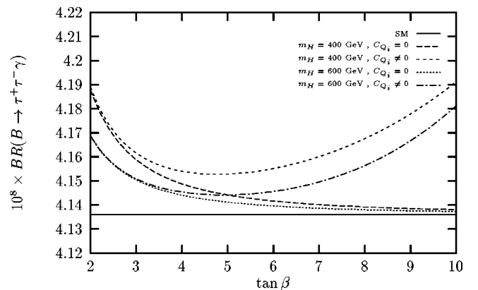
FIG. 3. Branching ratio as a function of \tan \beta in the SM and model I for different values of m_{H^\pm} . Curves with C_{Q_i} \neq 0 ( C_{Q_i} = 0 ) represent the contributions including (not including) the neutral Higgs boson interactions.
