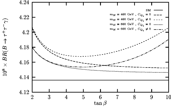
FIG. 4. The same as Fig. 3, but for model II.
