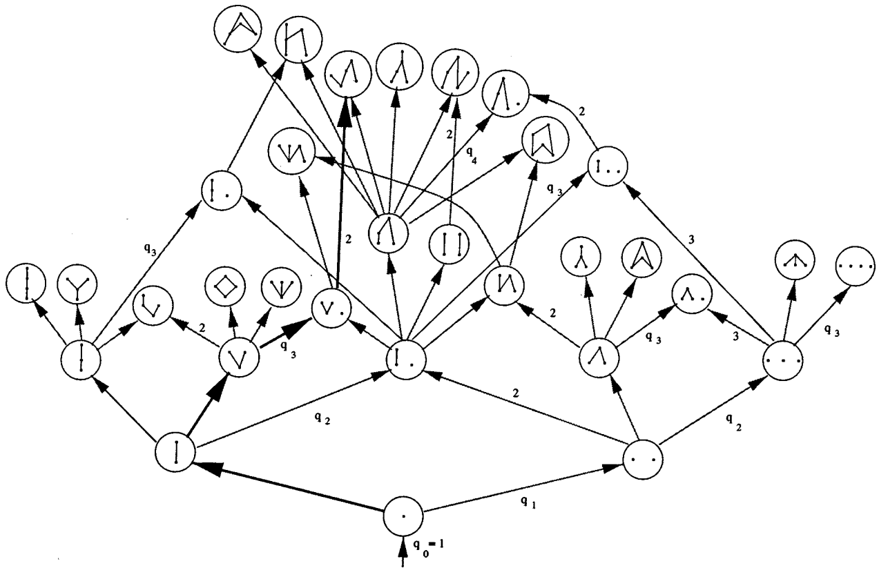
FIG. 1. The poset of finite causet.
