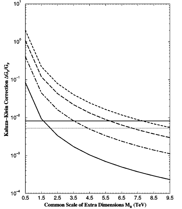
FIG. 1. Plot of the ratio (\Delta G_F^{\text{KK}}/G_F^{\text{SM}}) as a function of the common scale of extra dimension. The curves correspond to the case d=1 (solid), d=2 (dot-dashed), d=3 (long dashed), and d=4 (dashed). The horizontal solid line corresponds to the 2\sigma error on \Delta G_F^{\text{SM}}/G_F^{\text{SM}} while the horizontal dotted line is what the 2\sigma error will be if the error in the W boson measurements decreased by a factor of 2.
